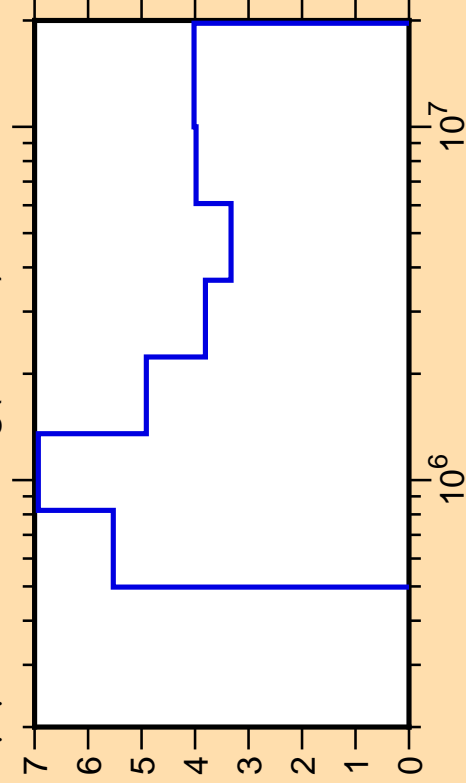
\Delta\mu/\mu vs. E for ^{24}\text{Mg}(\text{mt251})
