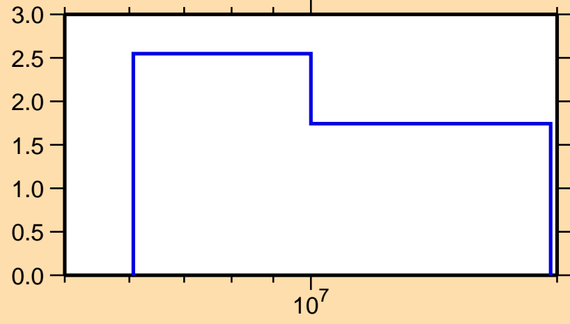
\Delta\sigma/\sigma vs. E for ^{24}\text{Mg}(n,n\text{onel.})
