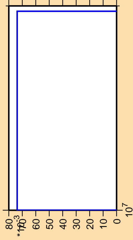
\Delta\sigma/\sigma vs. E for ^{24}\text{Mg}(n,\text{pd})
