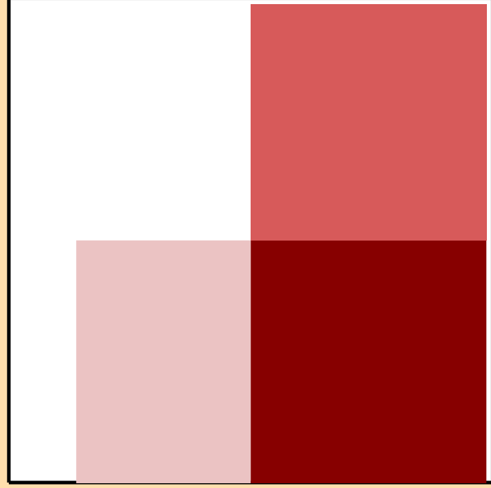
\Delta\sigma/\sigma vs. E for ^{24}\text{Mg}(n,ncont.)
