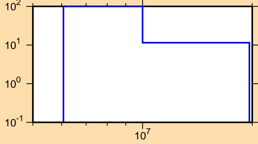
\Delta\sigma/\sigma vs. E for ^{24}\text{Mg}(n,n\text{cont.})
