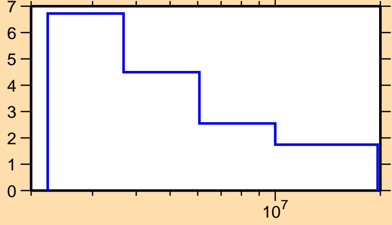
\Delta\sigma/\sigma vs. E for ^{24}\text{Mg}(n,\text{nonel.})
