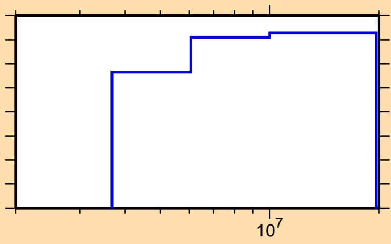
\sigma vs. E for ^{24}\text{Mg}(n,\alpha)
