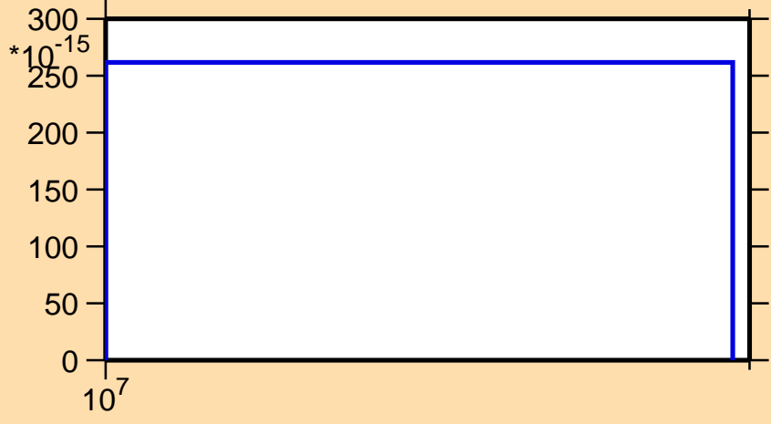
\sigma vs. E for ^{24}\text{Mg}(n,\text{pd})
