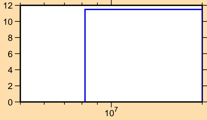
\Delta\sigma/\sigma vs. E for ^{24}\text{Mg}(n,ncont.)
