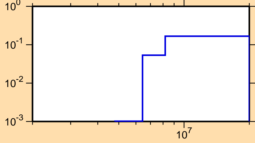
\sigma vs. E for ^{24}\text{Mg}(n,p)
