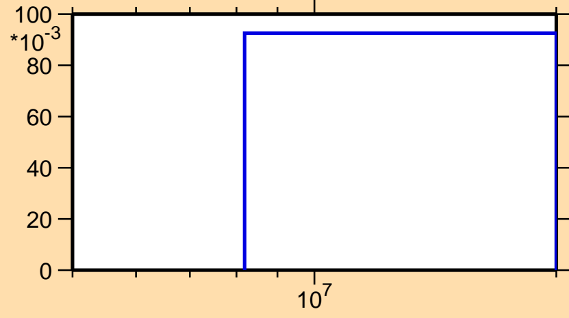
\sigma vs. E for ^{24}\text{Mg}(n,n\alpha)
