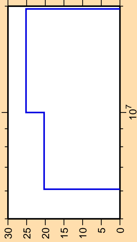
\Delta\sigma/\sigma vs. E for ^{25}\text{Mg}(n, ncont.)
