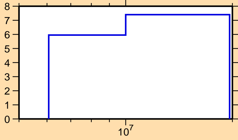
\Delta\sigma/\sigma vs. E for ^{25}\text{Mg}(n,n\text{onel.})
