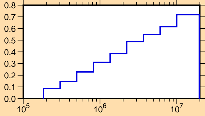
\mu vs. E for ^{26}\text{Mg}(\text{mt251})
