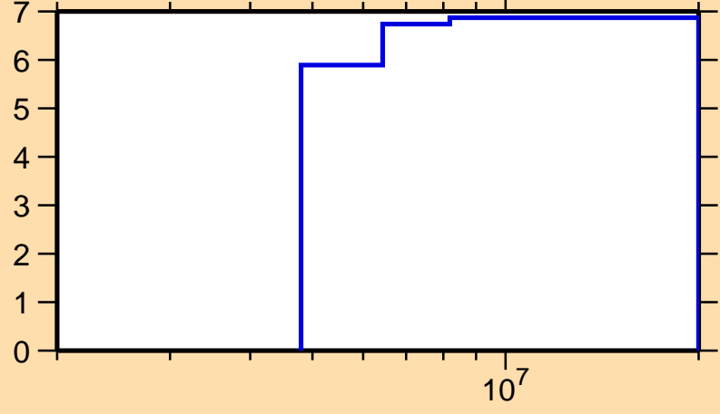
\Delta\sigma/\sigma vs. E for ^{26}\text{Mg}(n,\text{nonel.})
