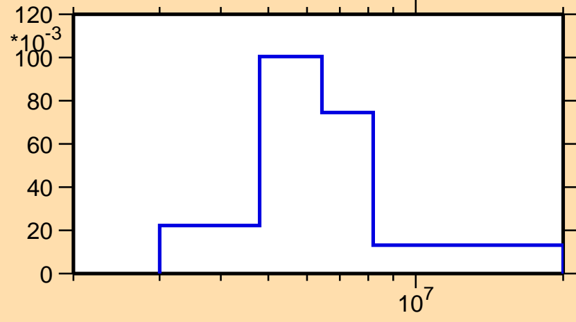
\sigma vs. E for ^{26}\text{Mg}(n,n_4)
