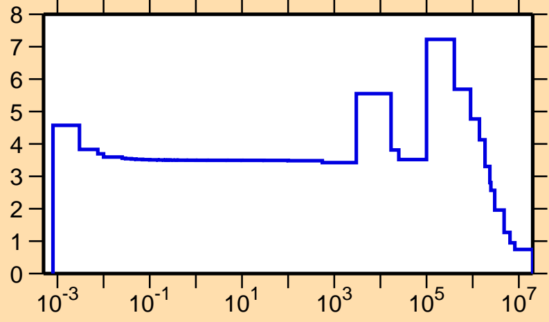
\sigma vs. E for ^{26}\text{Mg}(n,\text{el.})
