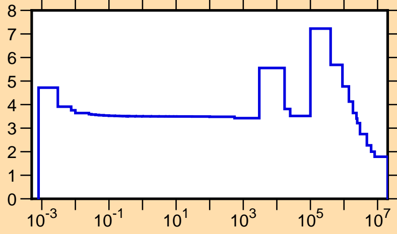
\sigma vs. E for ^{26}\text{Mg}(n,\text{tot.})
