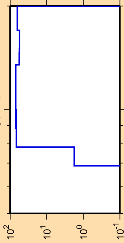
\Delta\sigma/\sigma vs. E for ^{28}\text{Mg}(n,\alpha)
