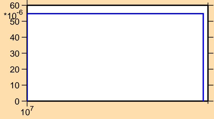
\sigma vs. E for ^{28}\text{Mg}(n,n\alpha)
