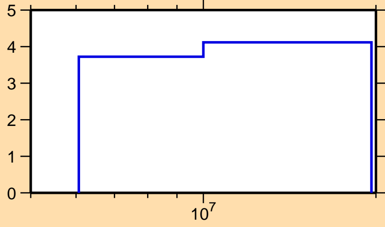
\Delta\sigma/\sigma vs. E for ^{28}\text{Mg}(n, n_{\text{nonel}})
