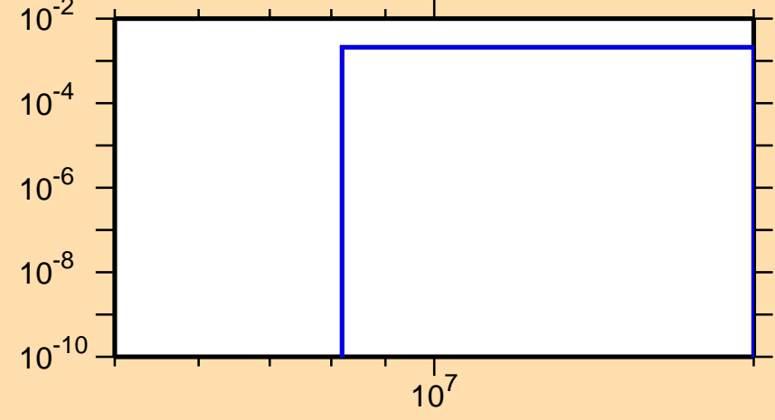
\sigma vs. E for ^{28}\text{Mg}(n,\alpha)
