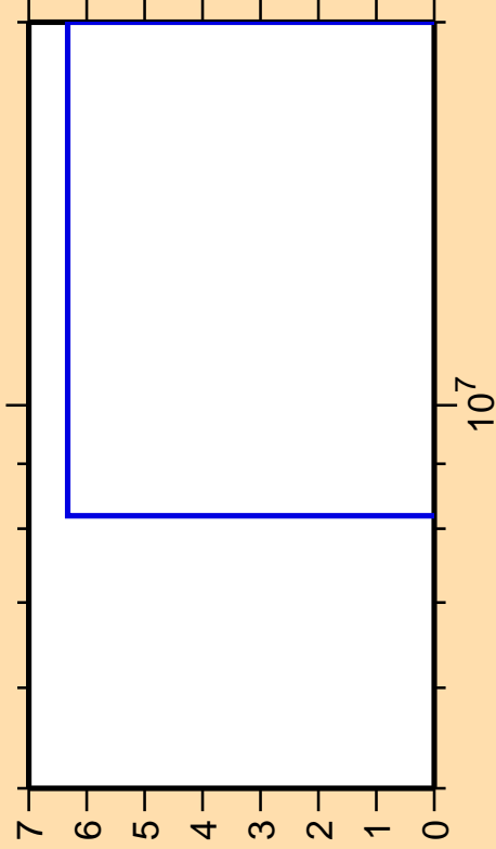
\Delta\sigma/\sigma vs. E for ^{28}\text{Mg}(n,2n)
