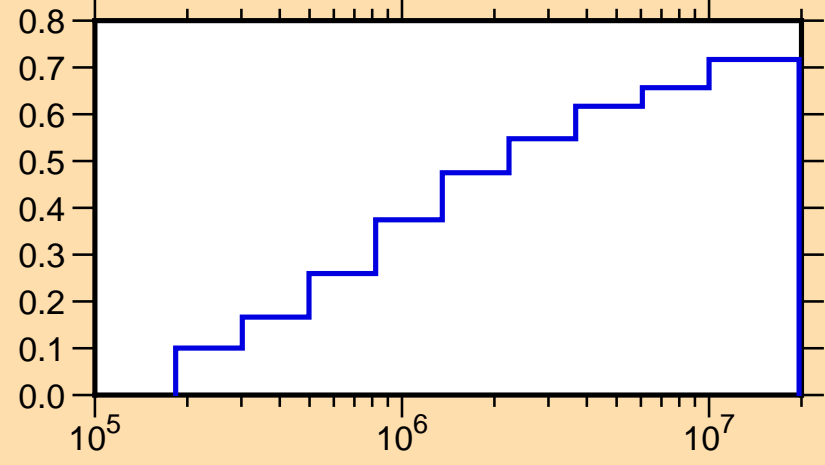
\mu vs. E for ^{29}\text{Mg}(\text{mt251})
