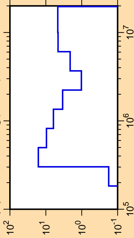
\Delta\mu/\mu vs. E for ^{29}\text{Mg}(\text{mt251})
