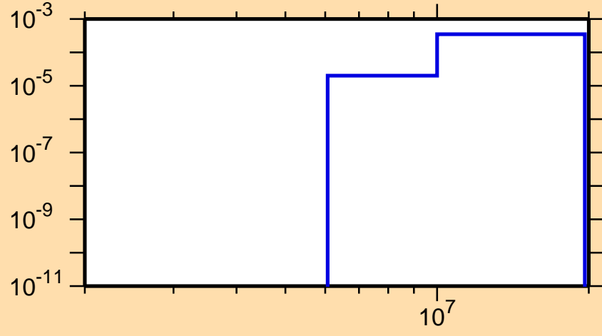
\sigma vs. E for ^{29}\text{Mg}(n,\alpha)
