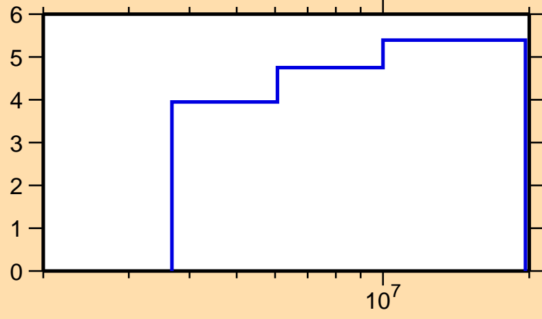
\Delta\sigma/\sigma vs. E for ^{29}\text{Mg}(n,n\text{onel.})
