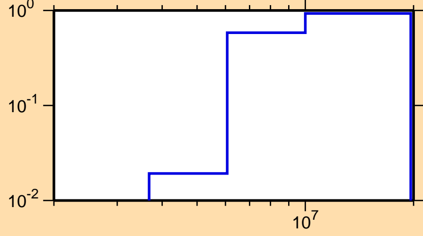
\sigma vs. E for ^{29}\text{Mg}(n,2n)
