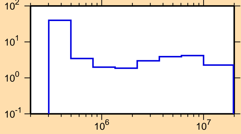
\Delta\sigma/\sigma vs. E for ^{29}\text{Mg}(n,\text{tot.})
