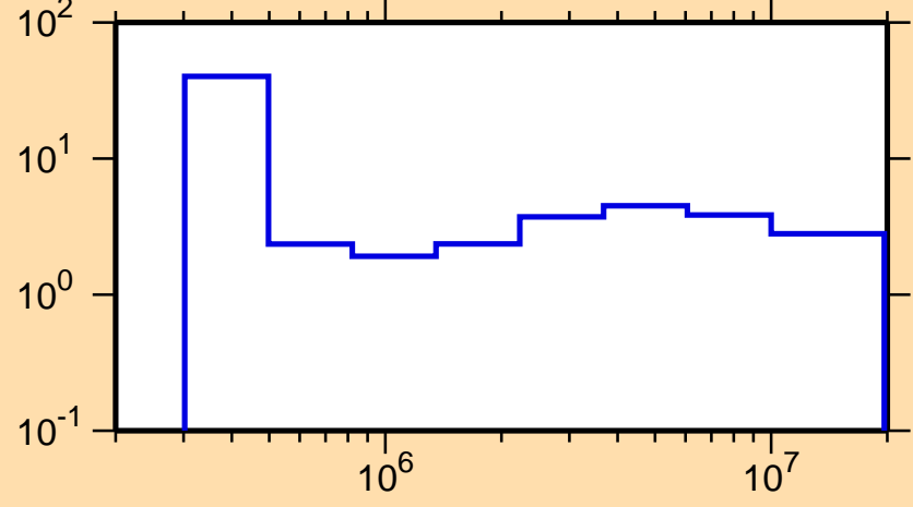
\Delta\sigma/\sigma vs. E for ^{29}\text{Mg}(n,\text{el.})
