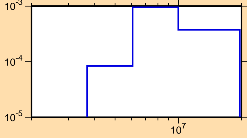
\sigma vs. E for ^{29}\text{Mg}(n,n\text{cont.})
