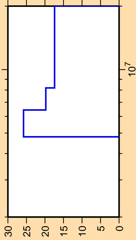
\Delta\sigma/\sigma vs. E for ^{29}\text{Mg}(n,\text{ncont.})
