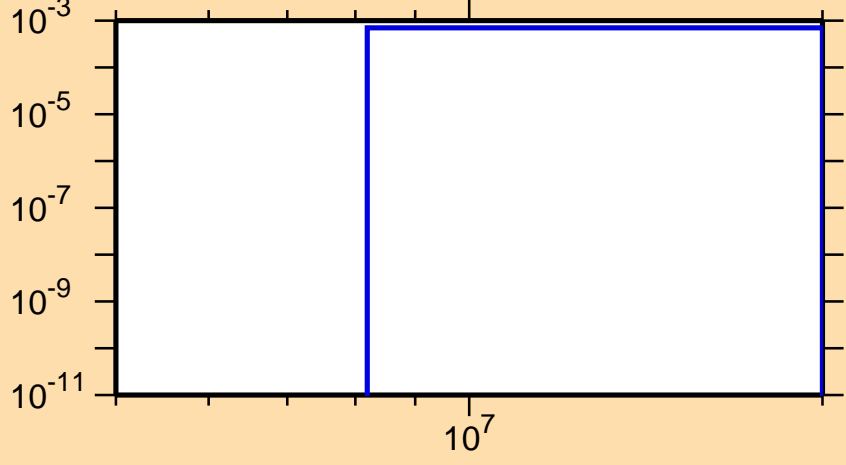
\sigma vs. E for ^{56}\text{Mn}(n,\alpha)
