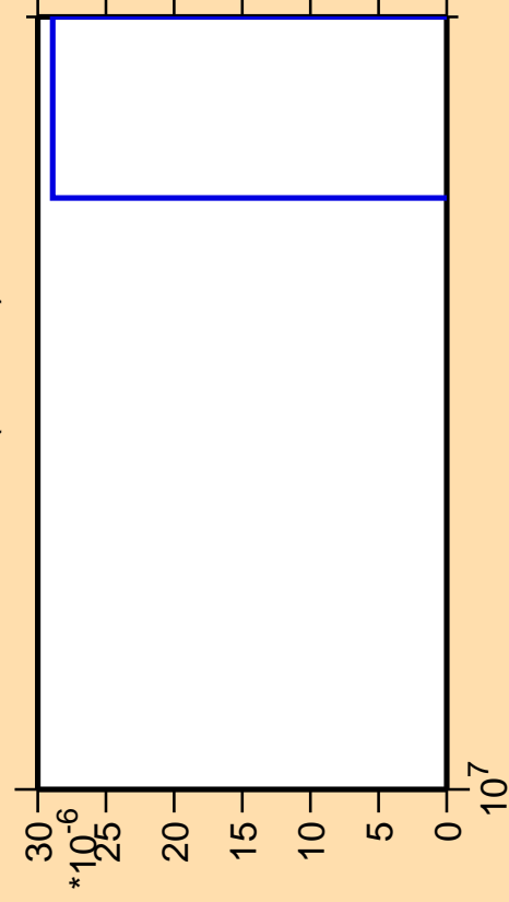
\Delta\sigma/\sigma vs. E for ^{59}\text{Mn}(n,\text{He}3)
