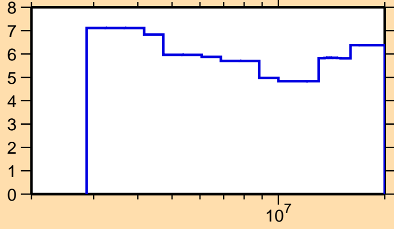
\Delta\sigma/\sigma vs. E for ^{59}\text{Mn}(n,n\text{onel.})
