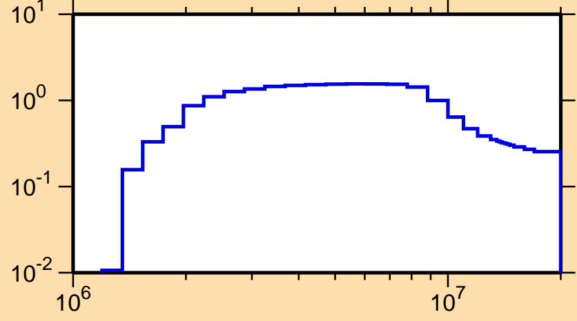
\sigma vs. E for ^{59}\text{Mn}(n,\text{inel.})
