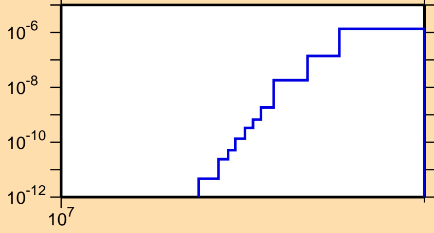
\sigma vs. E for ^{84}\text{Mo} (mt 45)
