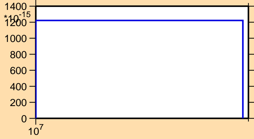
\sigma vs. E for ^{84}\text{Mo} (mt 34)
