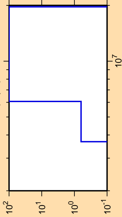
\Delta\sigma/\sigma vs. E for ^{84}\text{Mo}(n,\text{pd})
