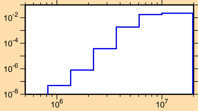
\sigma vs. E for ^{84}\text{Mo}(n,n\text{cont.})
