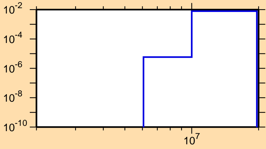
\sigma vs. E for ^{84}\text{Mo}(n,\text{pd})
