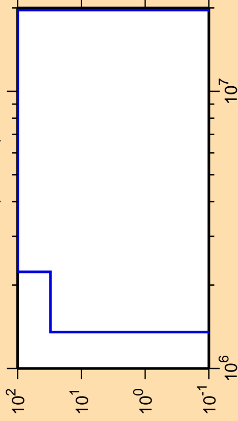
\Delta\sigma/\sigma vs. E for ^{84}\text{Mo}(n,\text{He3})
