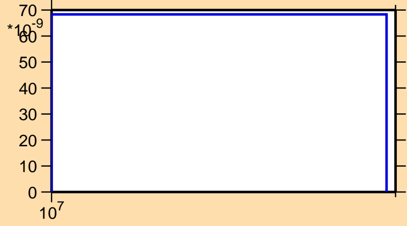
\sigma vs. E for ^{84}\text{Mo}(n,2n)
