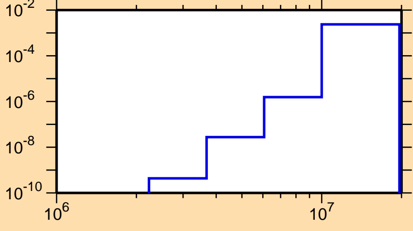
\sigma vs. E for ^{84}\text{Mo}(n,\text{He3})
