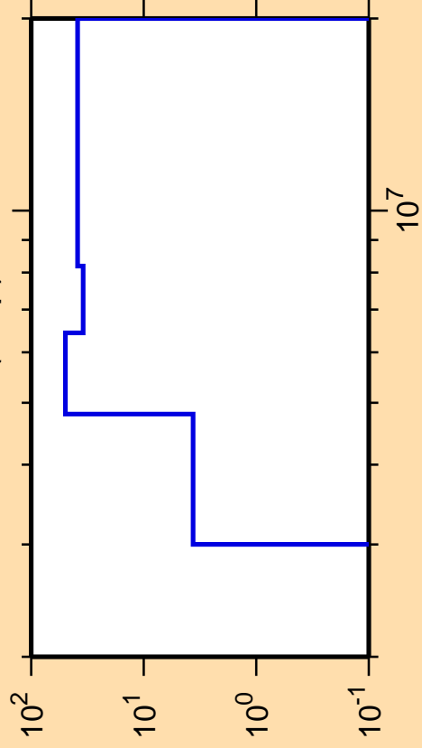
\Delta\sigma/\sigma vs. E for ^{84}\text{Mo}(n,np)
