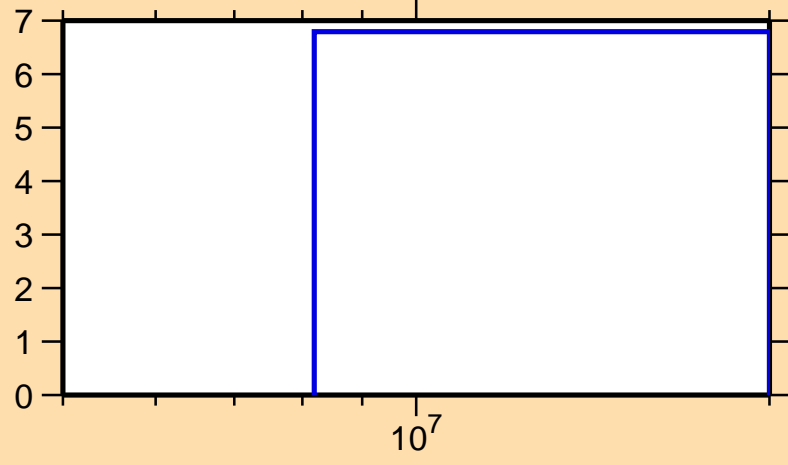
\Delta\sigma/\sigma vs. E for ^{84}\text{Mo}(n,\text{el.})
