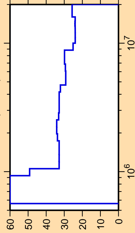
\Delta\sigma/\sigma vs. E for ^{86}\text{Mo}(n,\text{inel.})
