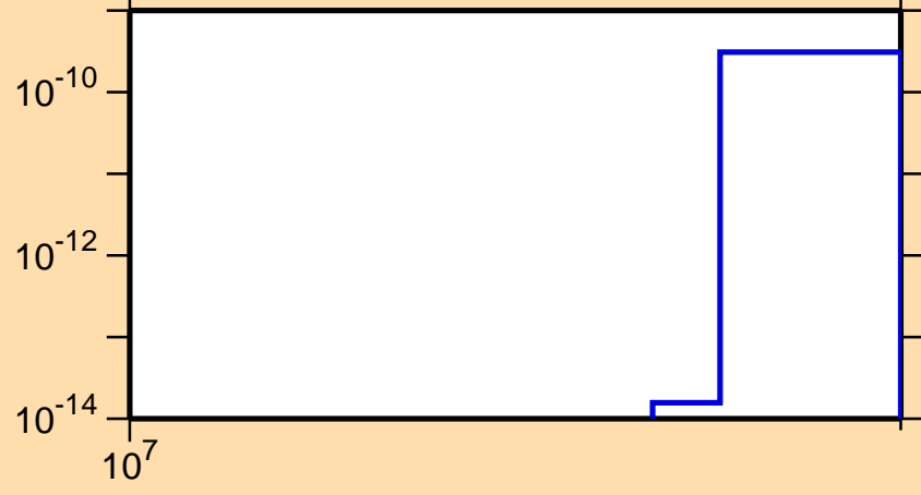
\sigma vs. E for ^{86}\text{Mo}(n,\text{nd})
