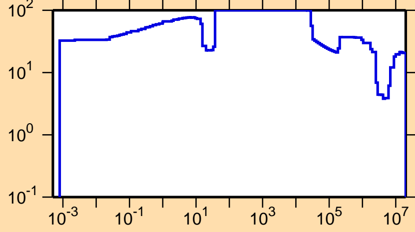
\Delta\sigma/\sigma vs. E for ^{86}\text{Mo}(n,\text{tot.})
