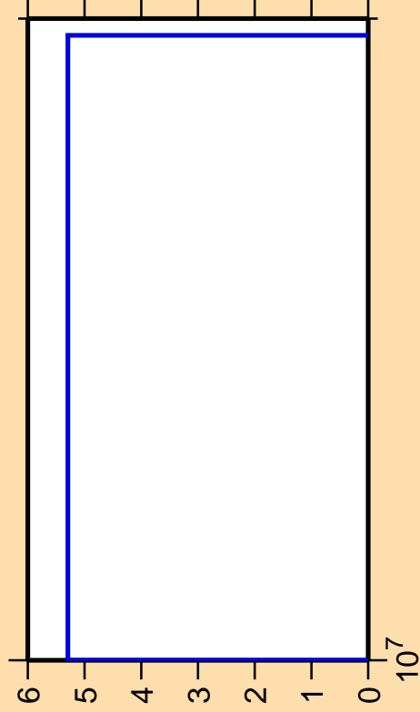
\Delta\sigma/\sigma vs. E for ^{86}\text{Mo}(n,nd)
