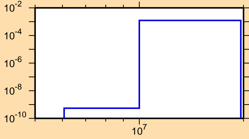
\sigma vs. E for ^{86}\text{Mo}(n,pd)
