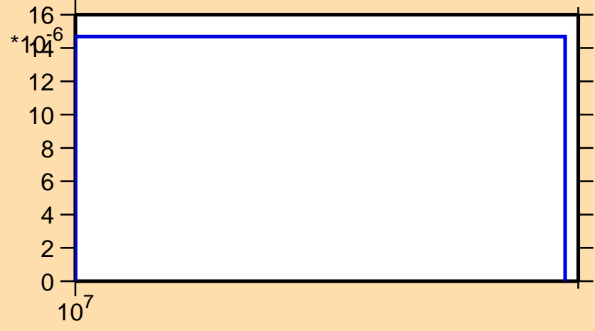
\sigma vs. E for ^{86}\text{Mo}(n,2n)
