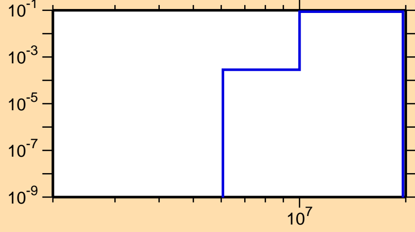
\sigma vs. E for ^{86}\text{Mo}(n,np)
