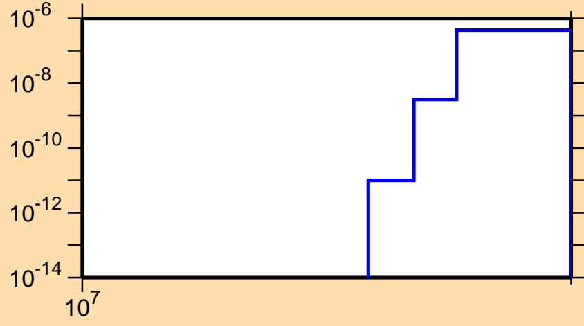
\sigma vs. E for ^{87}\text{Mo}(n,\text{nd})
