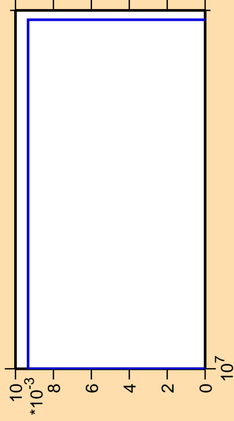
\Delta\sigma/\sigma vs. E for ^{87}\text{Mo}(n,2n\alpha)
