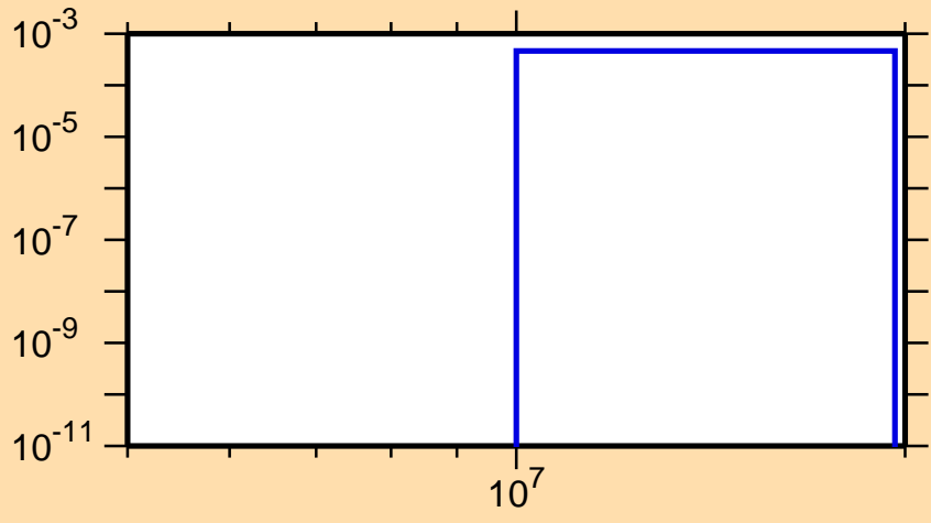
\sigma vs. E for ^{87}\text{Mo}(n,\text{pd})
