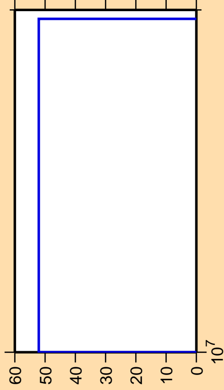
\Delta\sigma/\sigma vs. E for ^{87}\text{Mo}(n,n_1)
