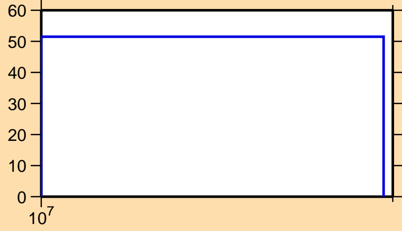
\Delta\sigma/\sigma vs. E for ^{87}\text{Mo}(n,\text{inel.})
