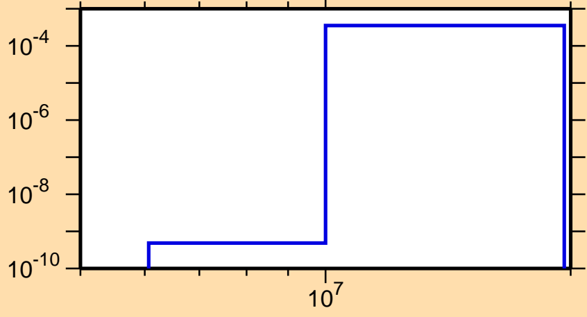
\sigma vs. E for ^{87}\text{Mo}(n,n\alpha)
