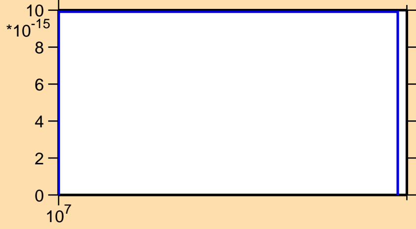
\sigma vs. E for ^{87}\text{Mo}(n,2n\alpha)
