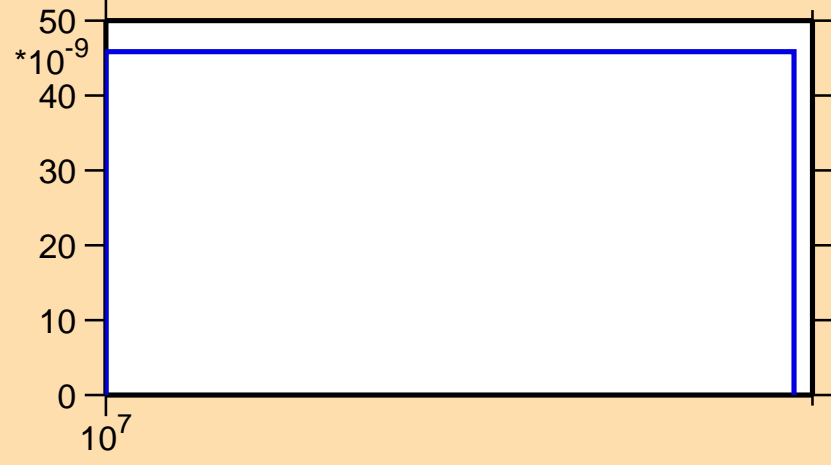
\sigma vs. E for ^{87}\text{Mo}(n,2np)
