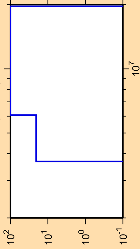
\Delta\sigma/\sigma vs. E for ^{87}\text{Mo}(n,\text{He}3)
