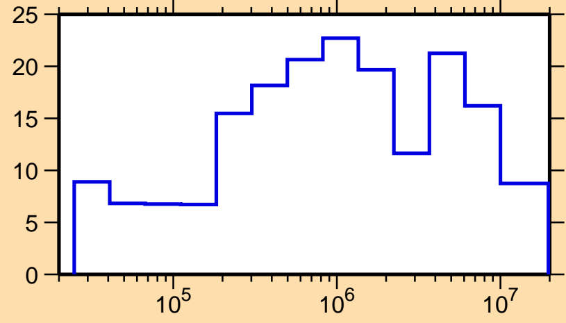
\Delta\sigma/\sigma vs. E for ^{87}\text{Mo}(n,\text{el.})
