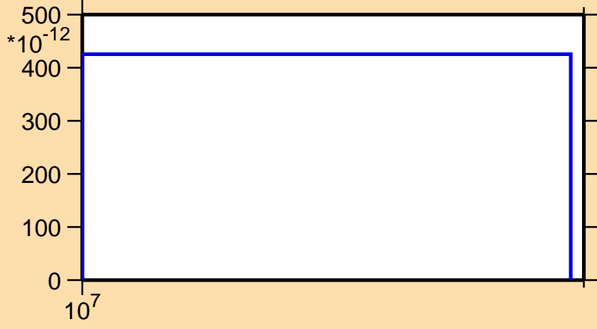
\sigma vs. E for ^{87}\text{Mo} (mt 34)
