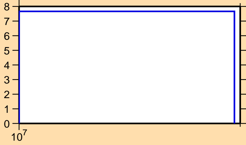
\Delta\sigma/\sigma vs. E for ^{87}\text{Mo}(n,\text{nonel.})
