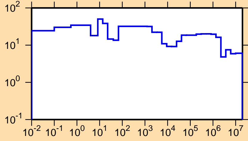
\Delta\sigma/\sigma vs. E for ^{87}\text{Mo}(n,\text{tot.})
