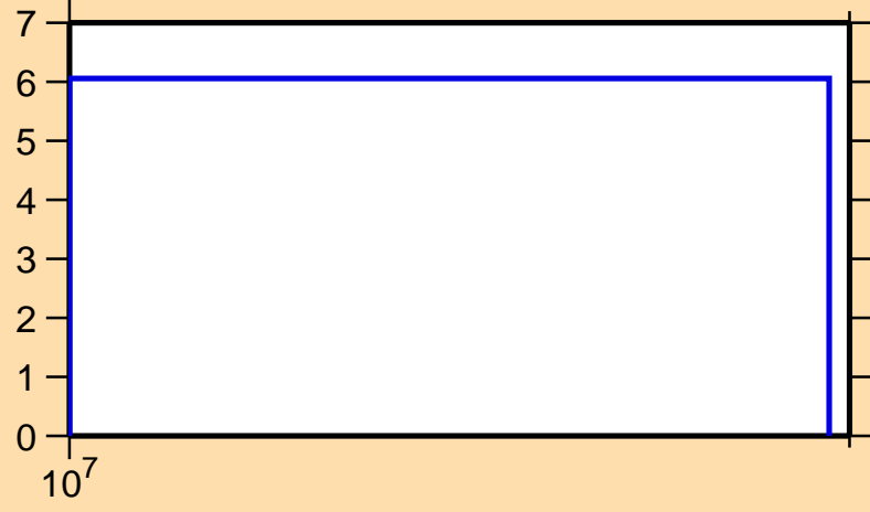
\Delta\sigma/\sigma vs. E for ^{87}\text{Mo}(n,\text{tot.})
