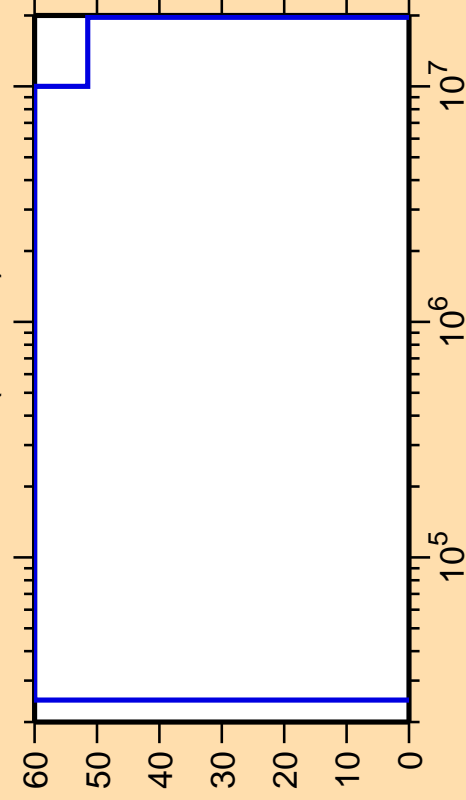
\Delta\sigma/\sigma vs. E for ^{87}\text{Mo}(n,\text{inel.})
