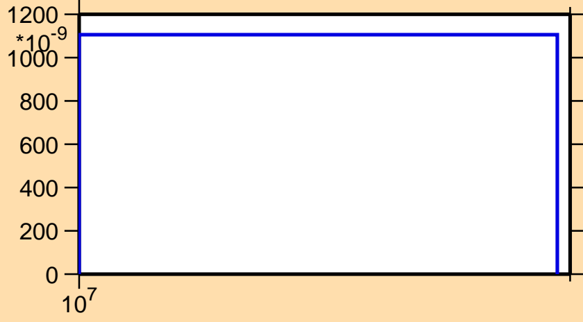
\sigma vs. E for ^{87}\text{Mo}(n,\text{pt})
