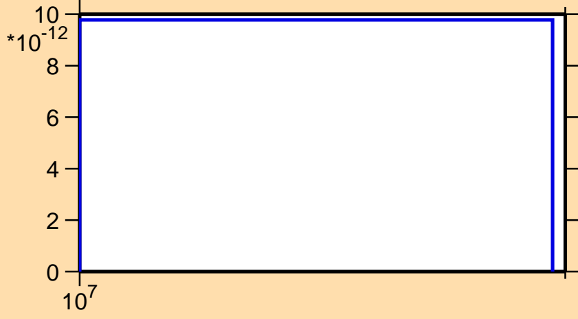
\sigma vs. E for ^{87}\text{Mo}(\text{mt117})
