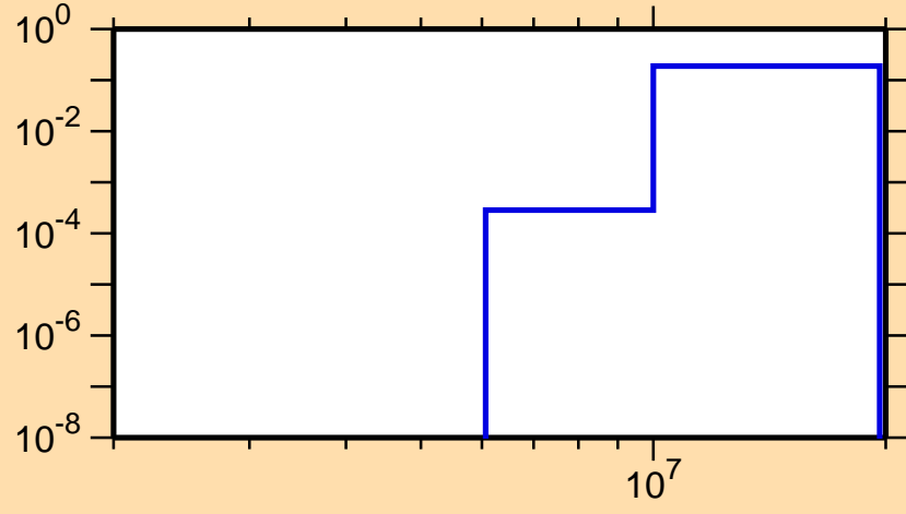
\sigma vs. E for ^{87}\text{Mo}(n,np)
