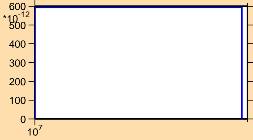
\sigma vs. E for ^{87}\text{Mo} (mt 45)
