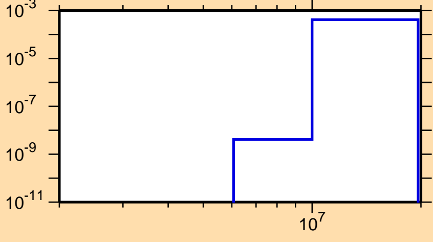
\sigma vs. E for ^{87}\text{Mo}(n,\text{He}3)
