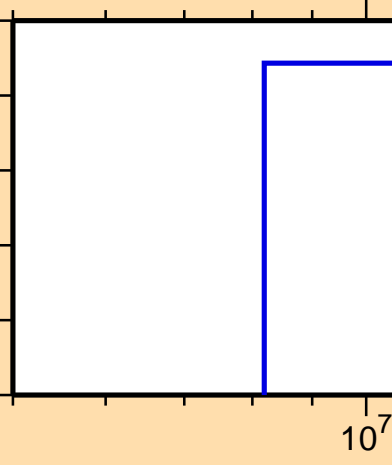
\sigma vs. E for ^{87}\text{Mo}(\text{mt117})
