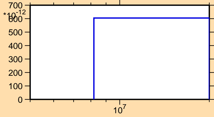
\sigma vs. E for ^{87}\text{Mo}(\text{mt } 45)
