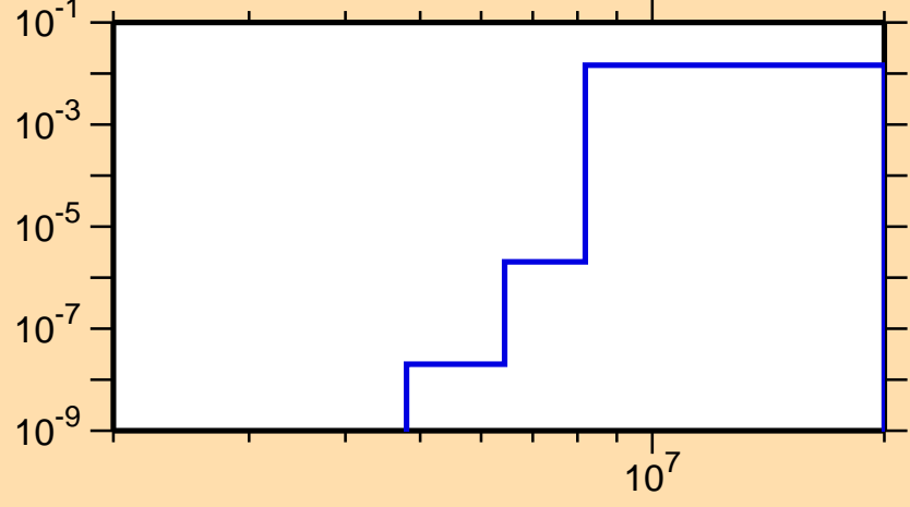
\sigma vs. E for ^{87}\text{Mo}(n,d)
