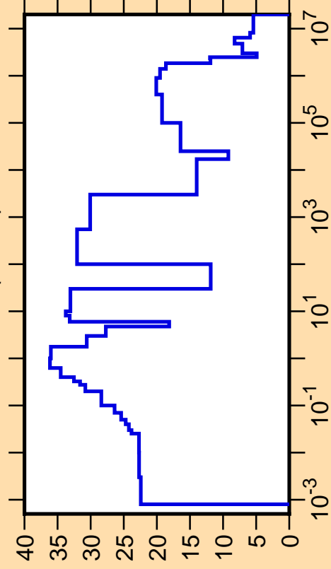
\Delta\sigma/\sigma vs. E for ^{87}\text{Mo}(n,\text{tot.})
