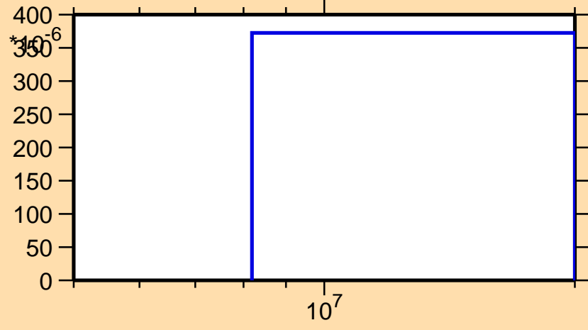
\sigma vs. E for ^{87}\text{Mo}(n,pd)
