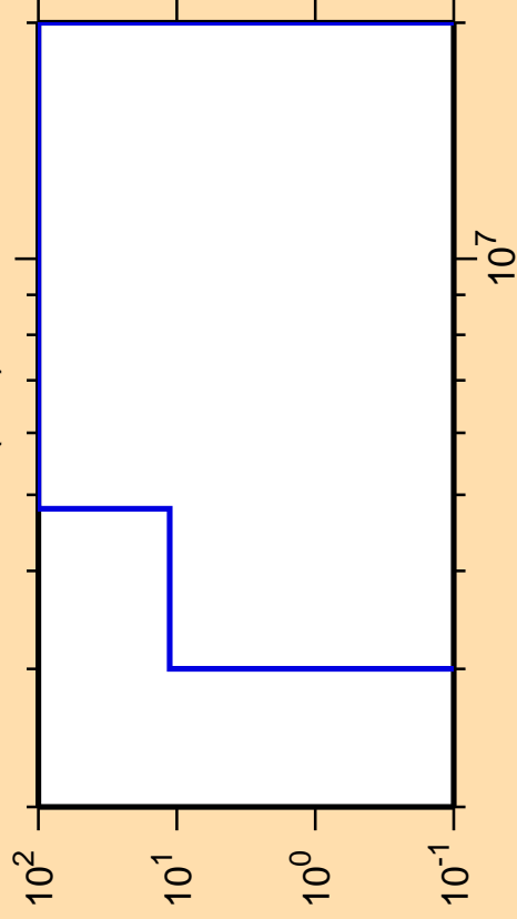
\Delta\sigma/\sigma vs. E for ^{87}\text{Mo}(n,d)
