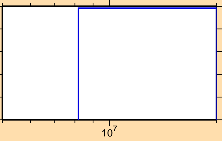
\sigma vs. E for ^{87}\text{Mo}(n,2n)
