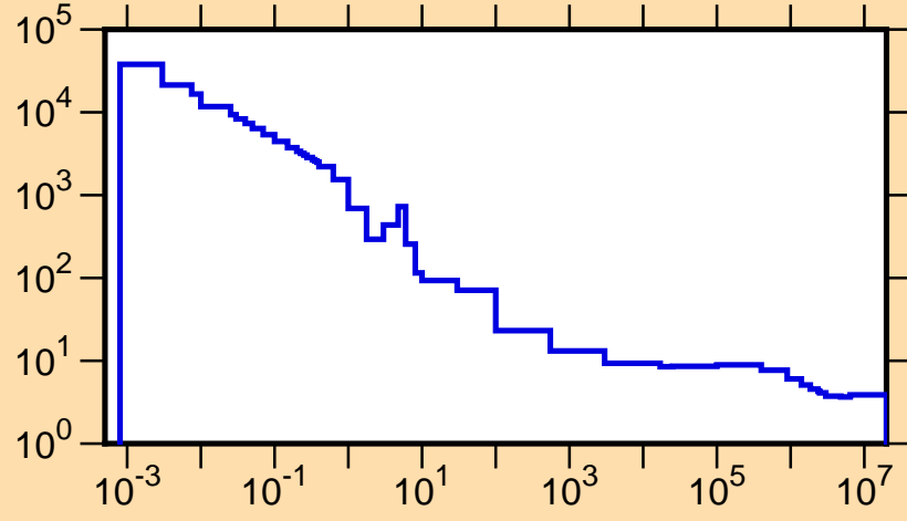
\sigma vs. E for ^{87}\text{Mo}(n,\text{tot.})
