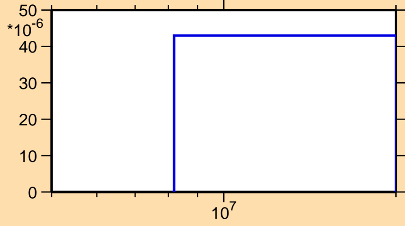
\sigma vs. E for ^{87}\text{Mo}(n,t)
