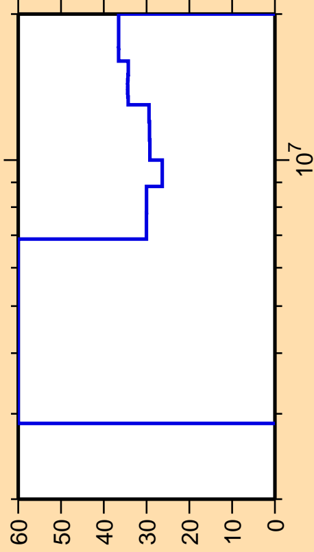
\Delta\sigma/\sigma vs. E for ^{88}\text{Mo}(n,\text{ncont.})
