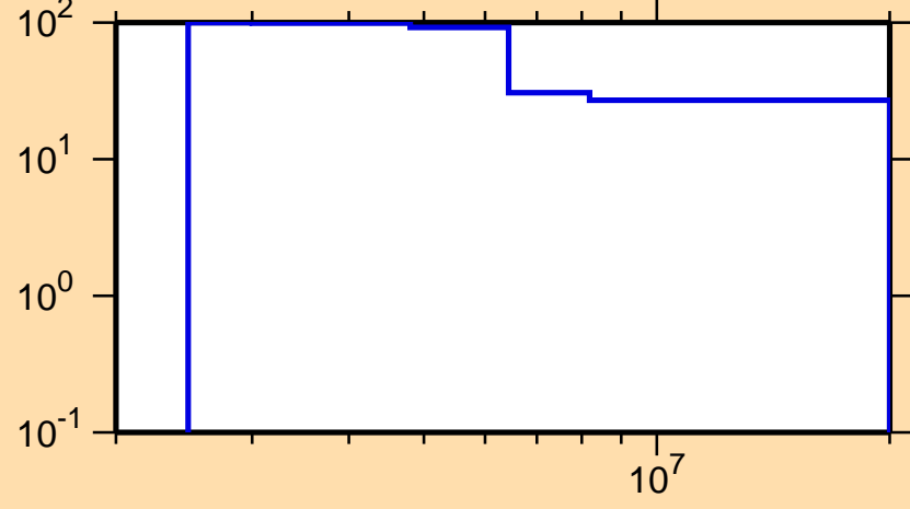
\Delta\sigma/\sigma vs. E for ^{88}\text{Mo}(n,n\text{cont.})
