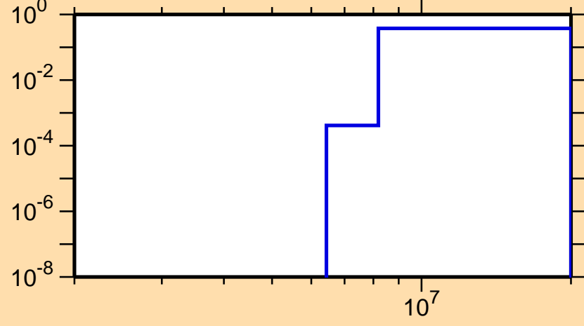
\sigma vs. E for ^{88}\text{Mo}(n,np)
