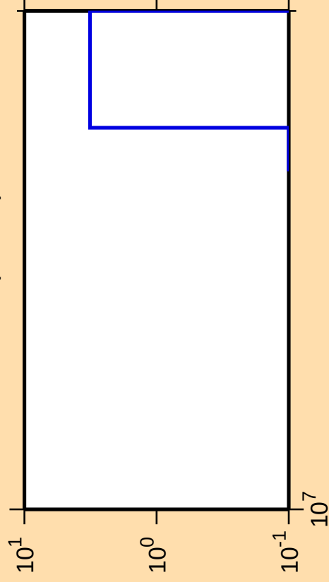
\Delta\sigma/\sigma vs. E for ^{89}\text{Mo}(n,2n\alpha)
