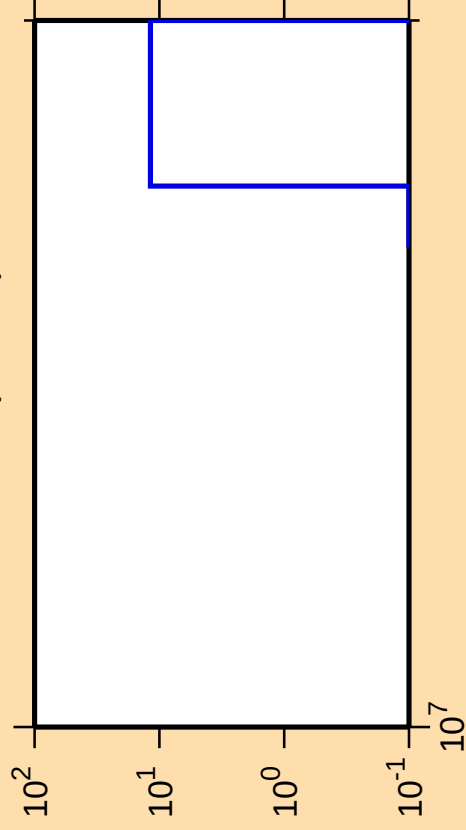
\Delta\sigma/\sigma vs. E for ^{89}\text{Mo}(\text{mt117})
