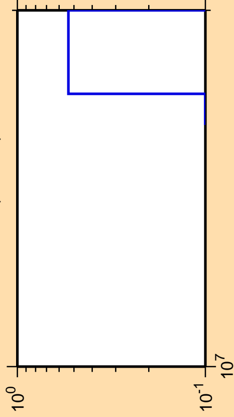
\Delta\sigma/\sigma vs. E for ^{91}\text{Mo}(\text{mt117})
