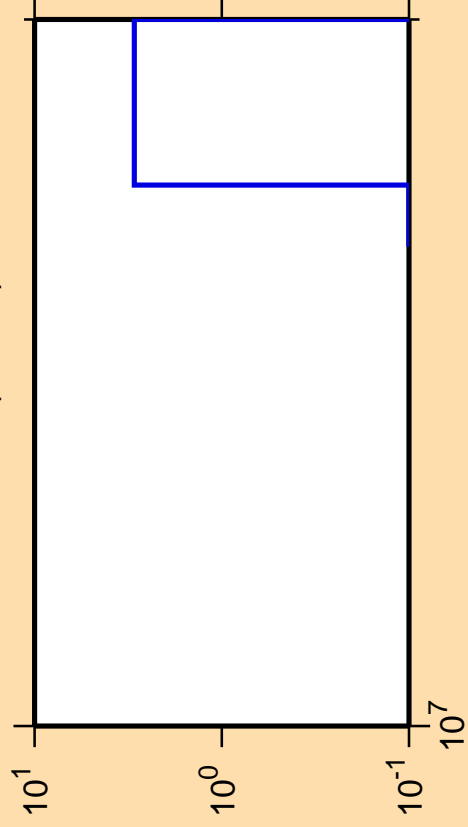
\Delta\sigma/\sigma vs. E for ^{91}\text{Mo}(\text{mt } 45)
