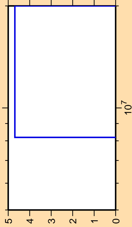
\Delta\sigma/\sigma vs. E for ^{91}\text{Mo}(\text{mt } 34)
