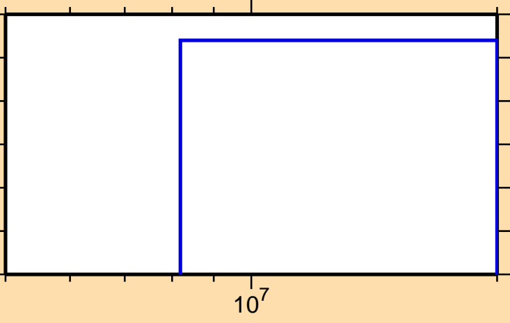
\sigma vs. E for ^{91}\text{Mo}(n,2n)
