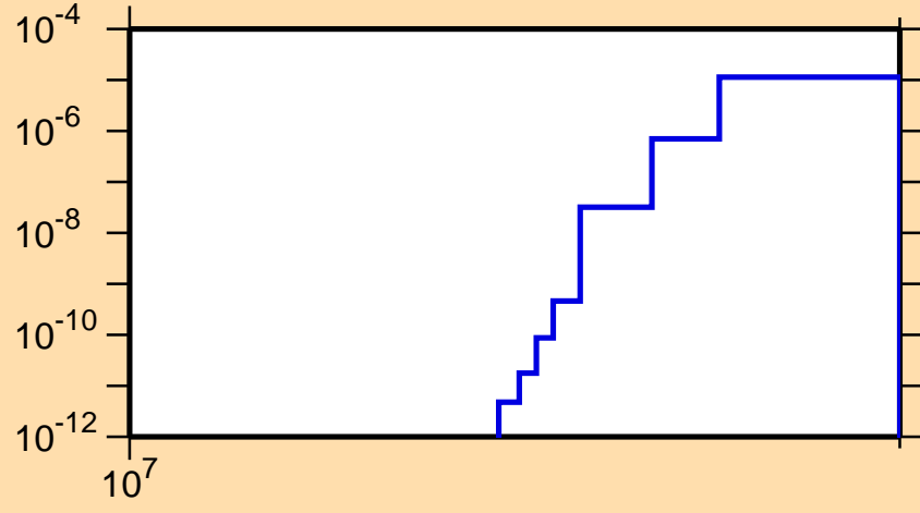
\sigma vs. E for ^{92}\text{Mo}(n,\text{pd})
