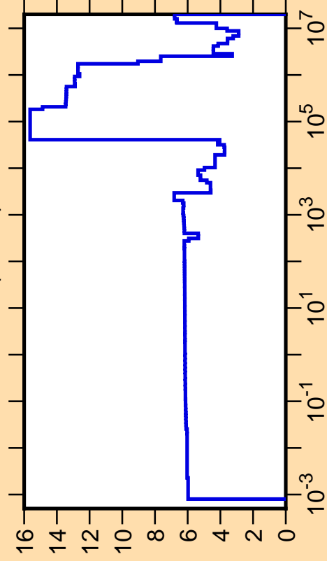
\Delta\sigma/\sigma vs. E for ^{92}\text{Mo}(n,\text{tot.})
