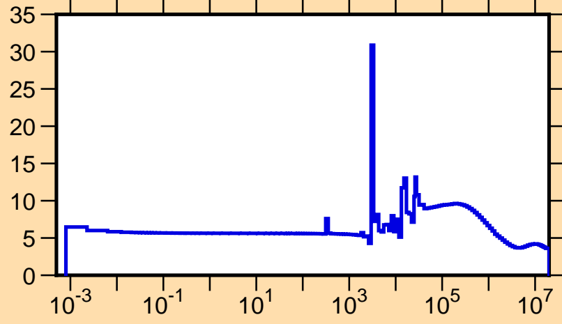
\sigma vs. E for ^{92}\text{Mo}(n,\text{tot.})
