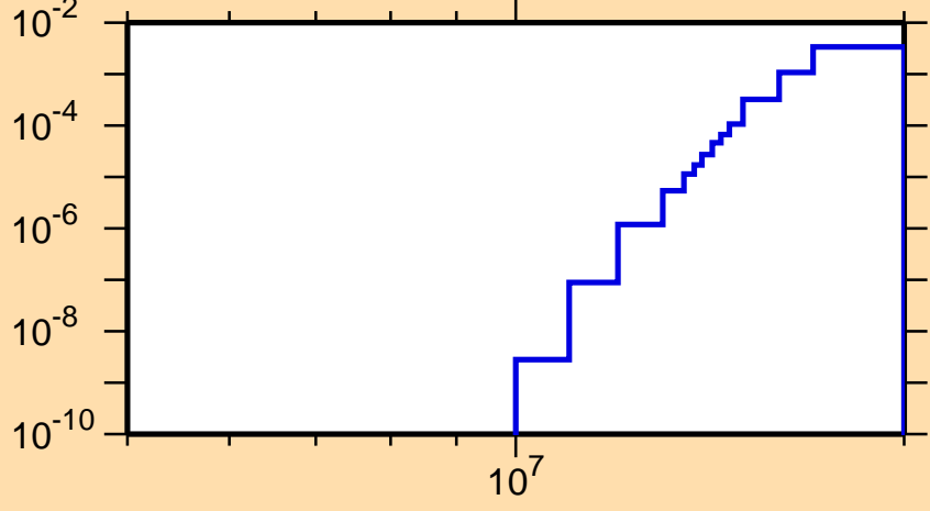
\sigma vs. E for ^{92}\text{Mo}(n,\alpha)
