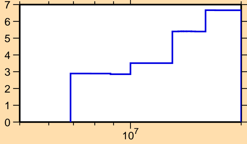
\Delta\sigma/\sigma vs. E for ^{95}\text{Mo}(n,\text{tot.})
