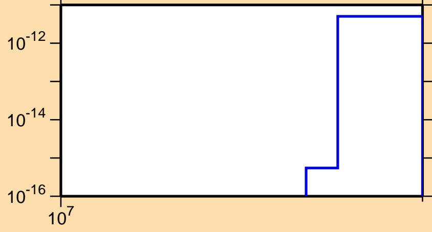
\sigma vs. E for ^{95}\text{Mo}(n,\text{pd})
