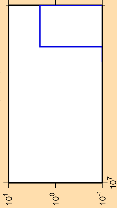
\Delta\sigma/\sigma vs. E for ^{95}\text{Mo} (mt 45)
