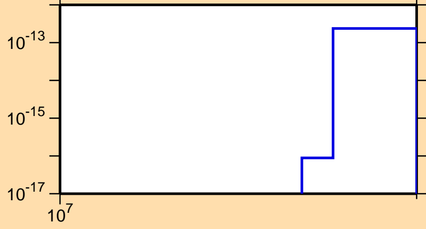
\sigma vs. E for ^{95}\text{Mo} (mt 34)
