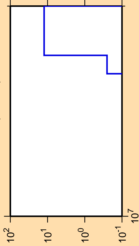
\Delta\sigma/\sigma vs. E for ^{95}\text{Mo}(\text{mt117})
