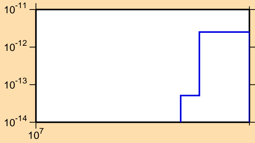
\sigma vs. E for ^{95}\text{Mo}(\text{mt117})
