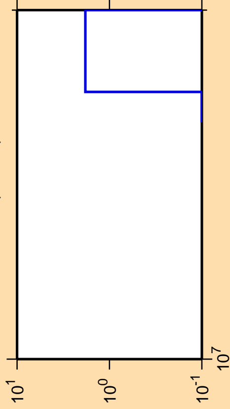
\Delta\sigma/\sigma vs. E for ^{95}\text{Mo} (mt 34)
