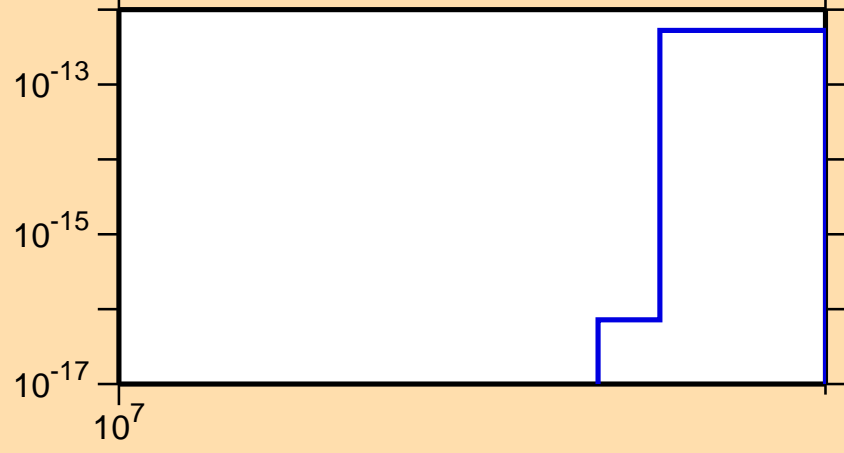
\sigma vs. E for ^{95}\text{Mo} (mt 45)
