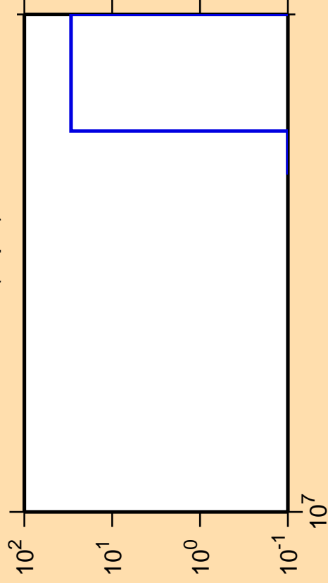
\Delta\sigma/\sigma vs. E for ^{95}\text{Mo}(n,\text{pd})
