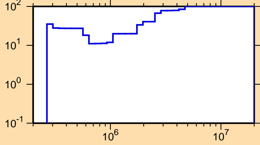
\Delta\sigma/\sigma vs. E for ^{97}\text{Mo}(n,n_1)
