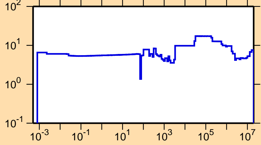
\Delta\sigma/\sigma vs. E for ^{97}\text{Mo}(n,\text{tot.})
