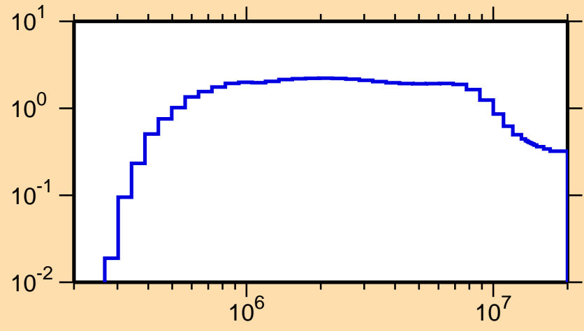
\sigma vs. E for ^{97}\text{Mo}(n,\text{inel.})
