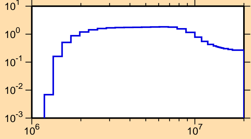
\sigma vs. E for ^{97}\text{Mo}(n,n\text{cont.})
