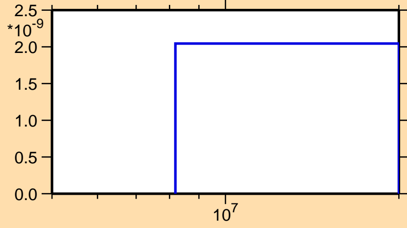
\sigma vs. E for ^{97}\text{Mo}(n,2np)
