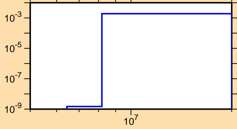
\sigma vs. E for ^{97}\text{Mo}(n,\alpha)
