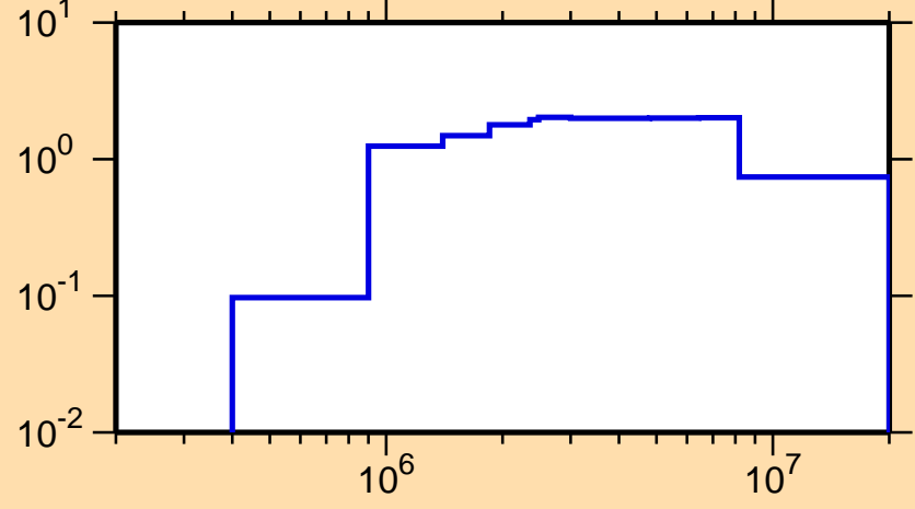
\sigma vs. E for ^{98}\text{Mo}(n,\text{inel.})
