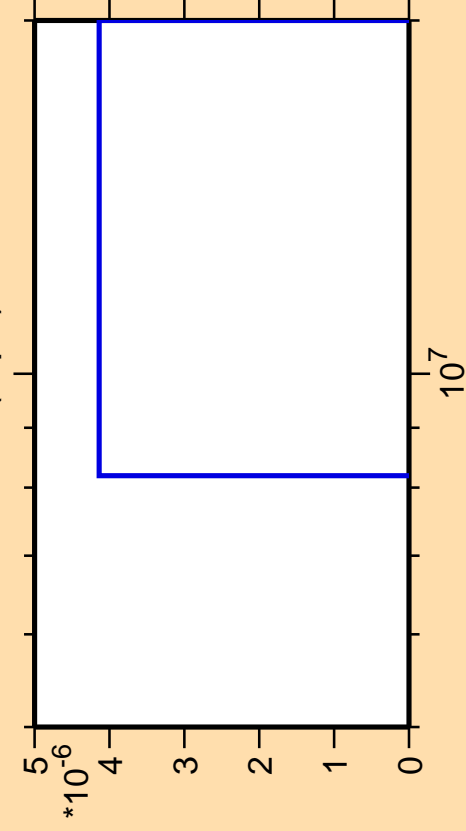
\Delta\sigma/\sigma vs. E for ^{98}\text{Mo}(n,pd)
