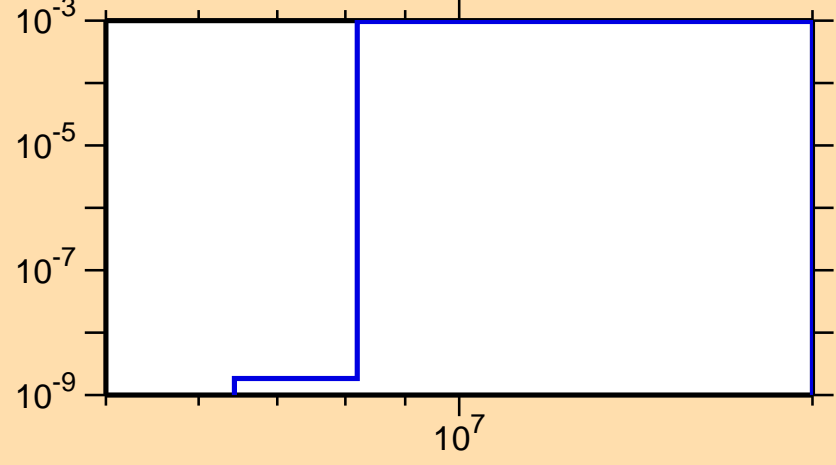
\sigma vs. E for ^{98}\text{Mo}(n,n\alpha)
