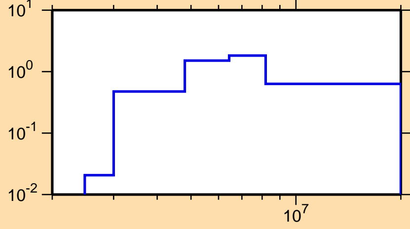
\sigma vs. E for ^{98}\text{Mo}(n,n\text{cont.})
