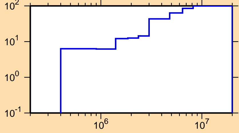
\Delta\sigma/\sigma vs. E for ^{98}\text{Mo}(n,n_1)
