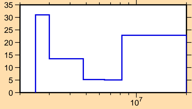
\Delta\sigma/\sigma vs. E for ^{98}\text{Mo}(n,n\text{cont.})
