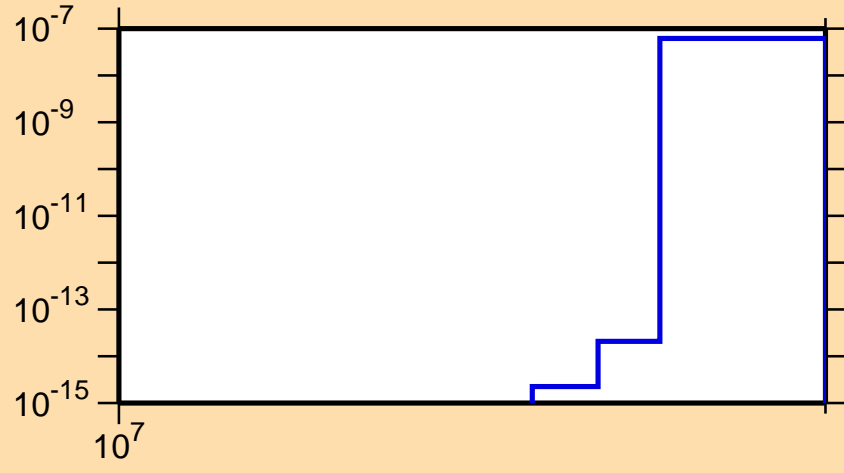
\sigma vs. E for ^{99}\text{Mo}(n,nt)
