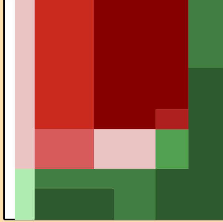
\Delta\sigma/\sigma vs. E for ^{99}\text{Mo}(n,2n)
