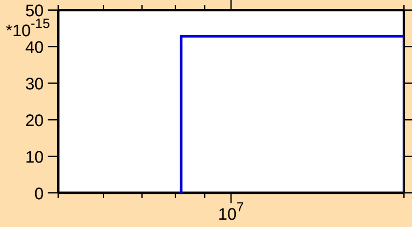
\sigma vs. E for ^{100}\text{Mo}(n,2np)
