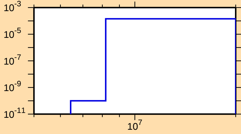
\sigma vs. E for ^{100}\text{Mo}(n,n\alpha)
