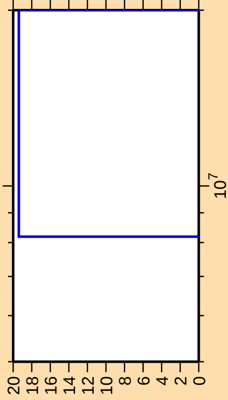
\Delta\sigma/\sigma vs. E for ^{100}\text{Mo}(n,n_1)
