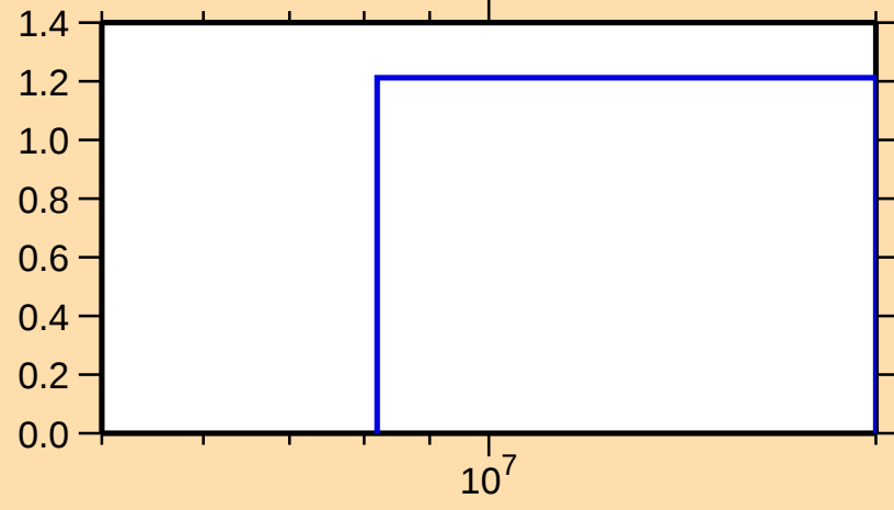
\sigma vs. E for ^{100}\text{Mo}(n,2n)
