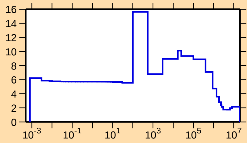
\sigma vs. E for ^{100}\text{Mo}(n,\text{el.})
