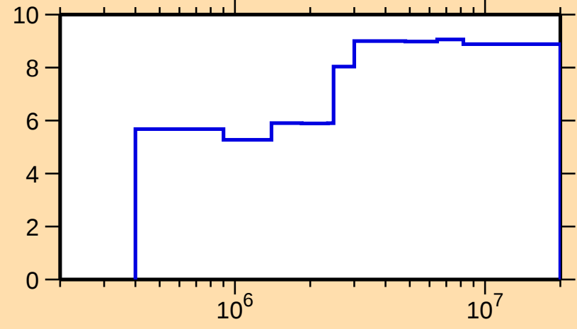
\Delta\sigma/\sigma vs. E for ^{100}\text{Mo}(\text{n,nonel.})
