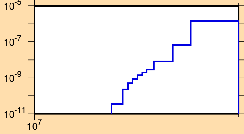
\sigma vs. E for ^{101}\text{Mo}(n,2n\alpha)
