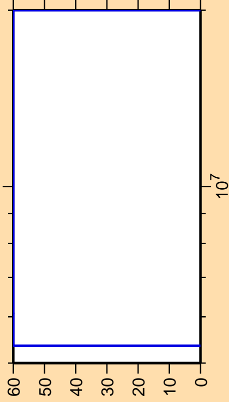
\Delta\sigma/\sigma vs. E for ^{101}\text{Mo}(n,p)
