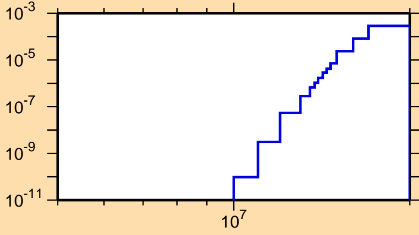
\sigma vs. E for ^{102}\text{Mo}(n,\alpha)
