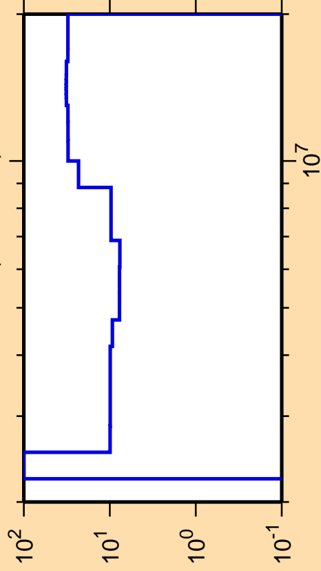
\Delta\sigma/\sigma vs. E for ^{102}\text{Mo}(n,\text{ncont.})
