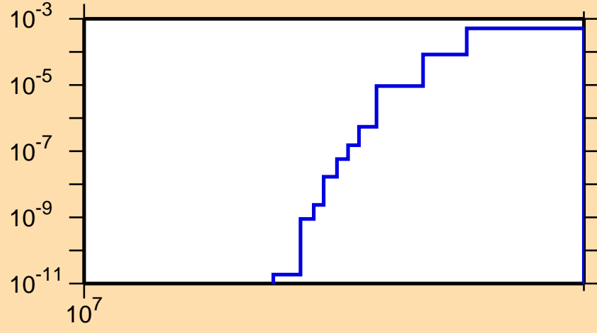
\sigma vs. E for ^{102}\text{Mo}(n,np)
