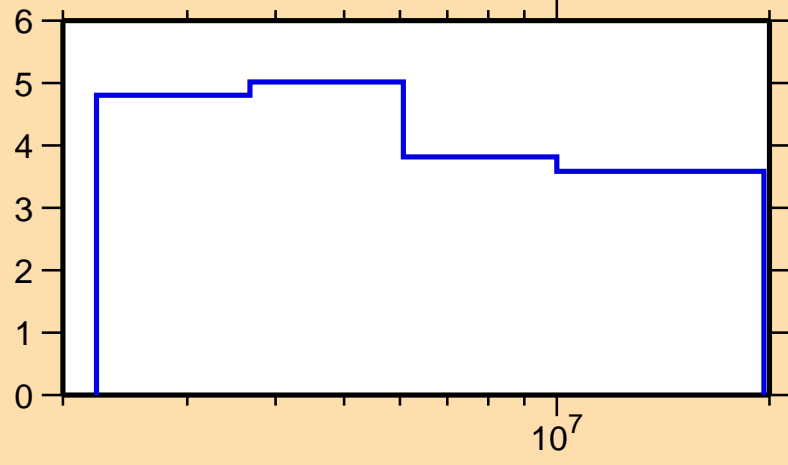
\Delta\sigma/\sigma vs. E for ^{102}\text{Mo}(n,n\text{onel.})
