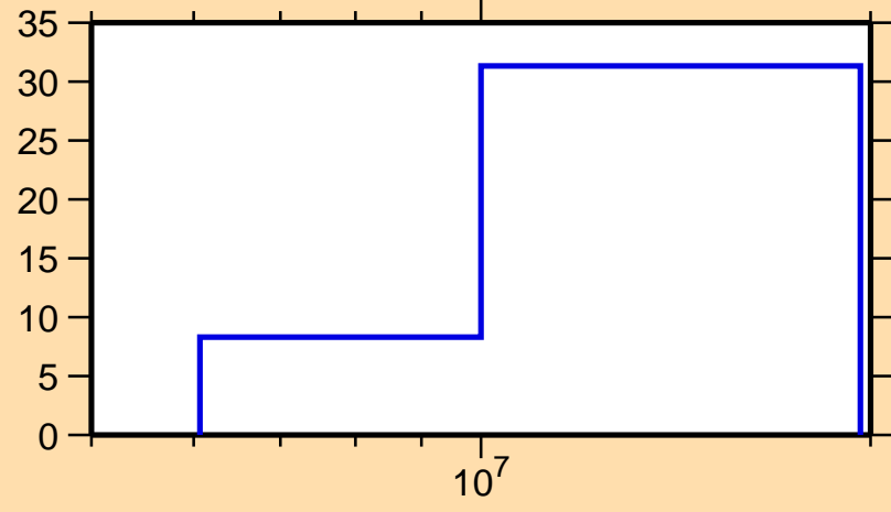
\Delta\sigma/\sigma vs. E for ^{102}\text{Mo}(n,ncont.)
