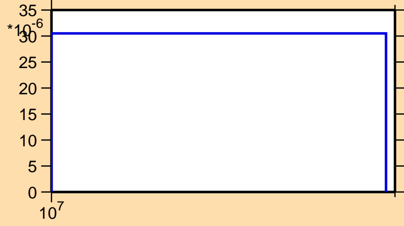
\sigma vs. E for ^{102}\text{Mo}(n,d)
