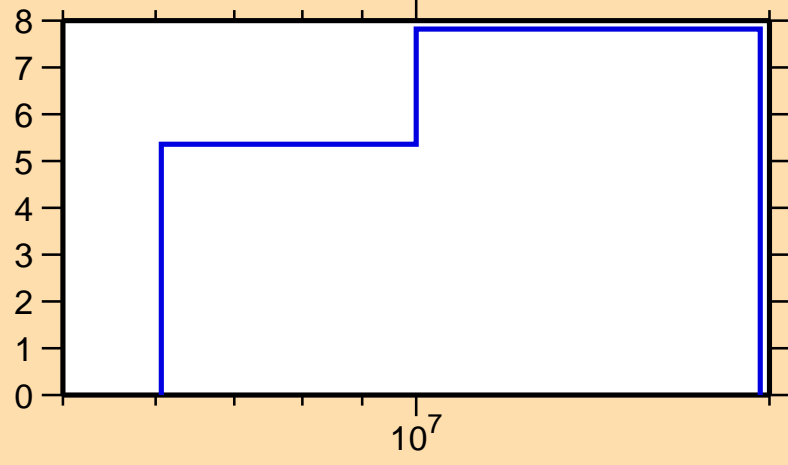
\Delta\sigma/\sigma vs. E for ^{102}\text{Mo}(n,el.)
