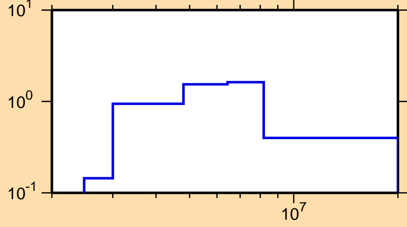
\sigma vs. E for ^{102}\text{Mo}(n,n\text{cont.})
