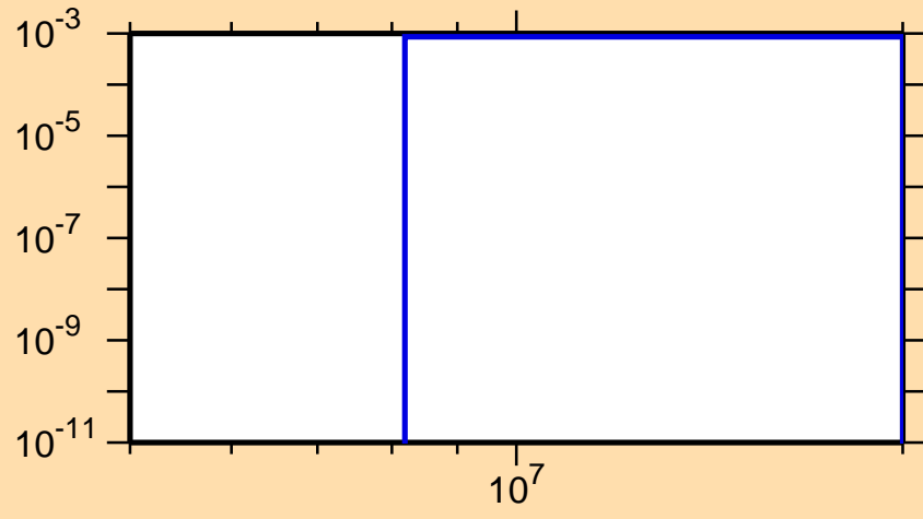
\sigma vs. E for ^{102}\text{Mo}(n,p)
