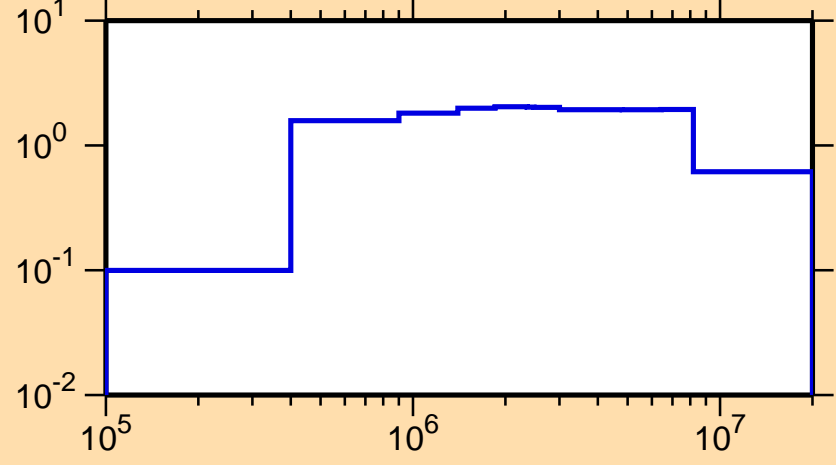
\sigma vs. E for ^{102}\text{Mo}(n,\text{inel.})
