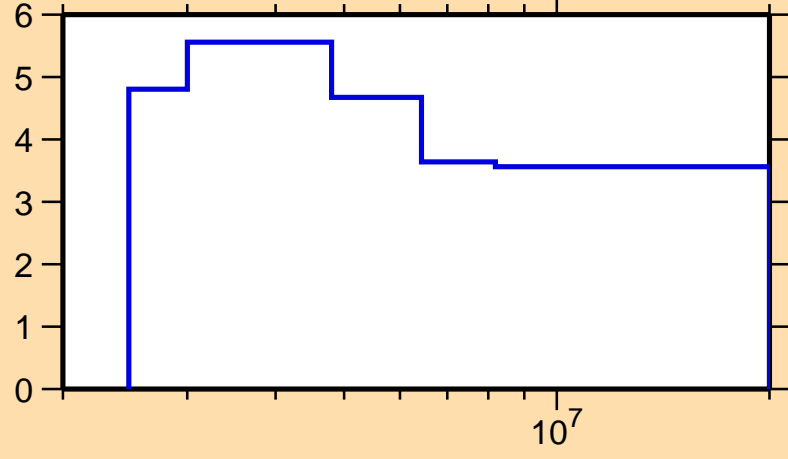
\Delta\sigma/\sigma vs. E for ^{102}\text{Mo}(n,\text{nonel.})
