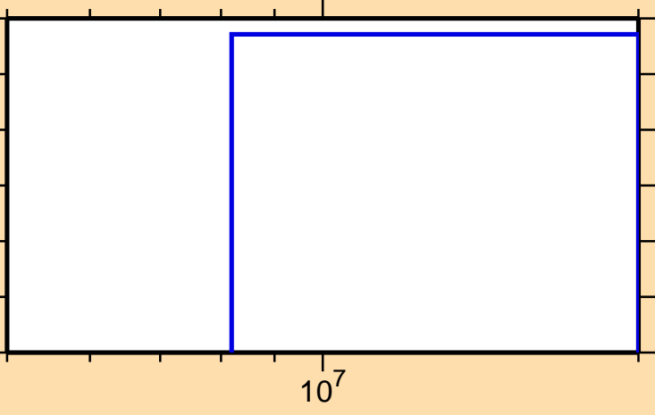
\sigma vs. E for ^{102}\text{Mo}(n,\text{nd})
