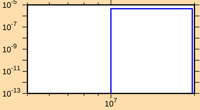
\sigma vs. E for ^{103}\text{Mo}(n,t)
