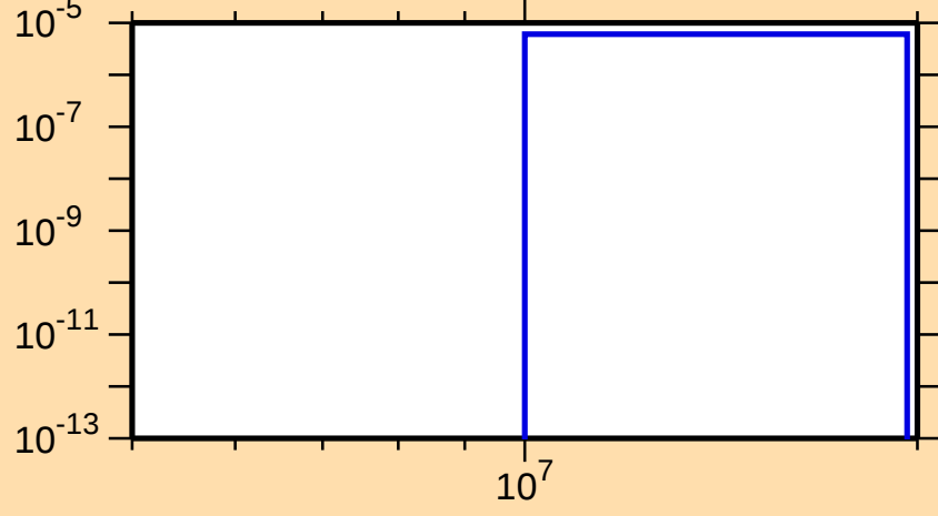
\sigma vs. E for ^{103}\text{Mo}(n,n\alpha)
