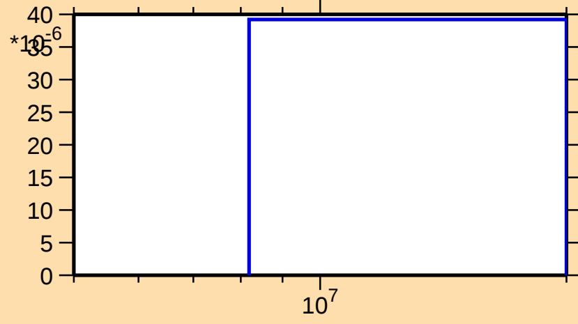
\sigma vs. E for ^{103}\text{Mo}(n,d)
