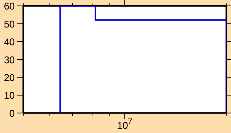
\Delta\sigma/\sigma vs. E for ^{103}\text{Mo}(n,\gamma)
