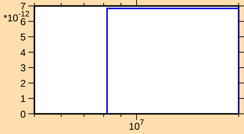
\sigma vs. E for ^{103}\text{Mo}(n,nt)
