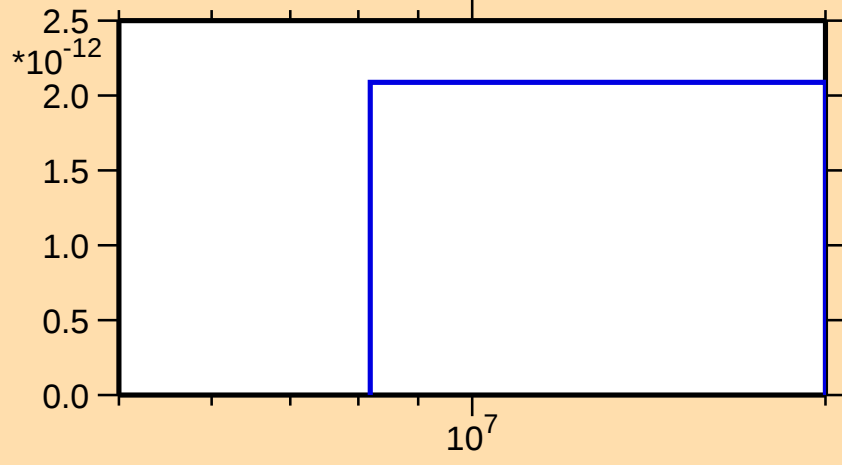
\sigma vs. E for ^{103}\text{Mo}(n,2np)
