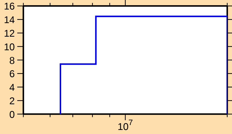
\Delta\sigma/\sigma vs. E for ^{103}\text{Mo}(n,\text{el.})
