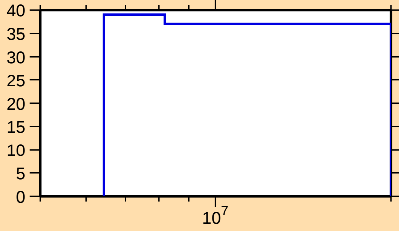
\Delta\sigma/\sigma vs. E for ^{103}\text{Mo}(n,2n)
