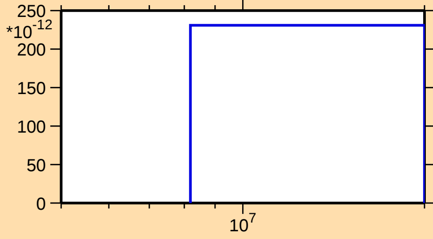
\sigma vs. E for ^{103}\text{Mo}(n,2n\alpha)
