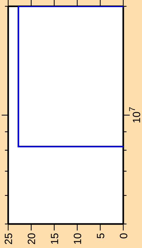
\Delta\sigma/\sigma vs. E for ^{103}\text{Mo}(n,nt)
