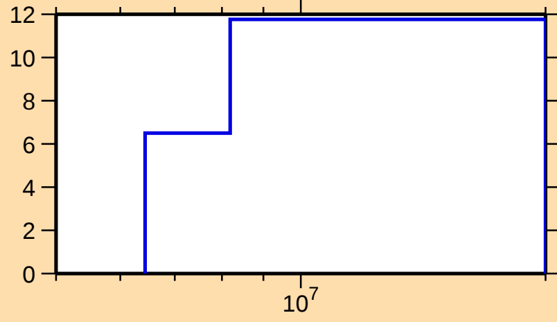
\Delta\sigma/\sigma vs. E for ^{103}\text{Mo}(n,\text{tot.})
