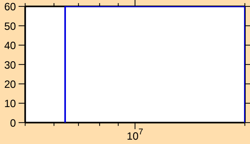
\Delta\sigma/\sigma vs. E for ^{103}\text{Mo}(n,n\text{cont.})
