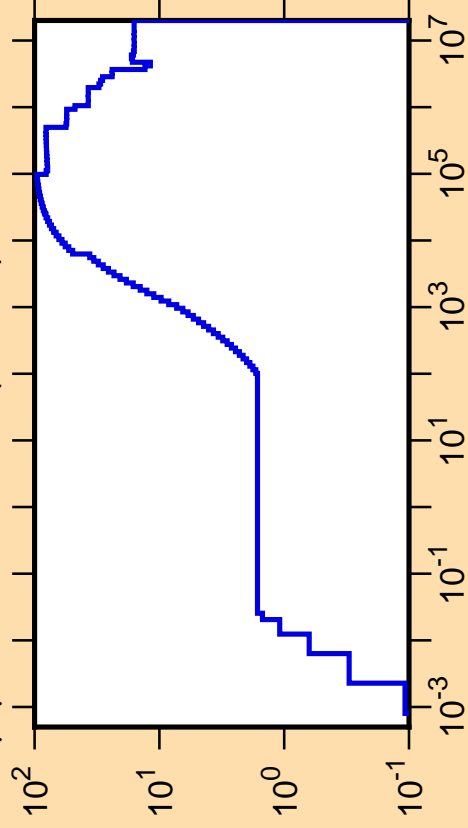
\Delta\mu/\mu vs. E for ^{105}\text{Mo}(\text{mt251})
