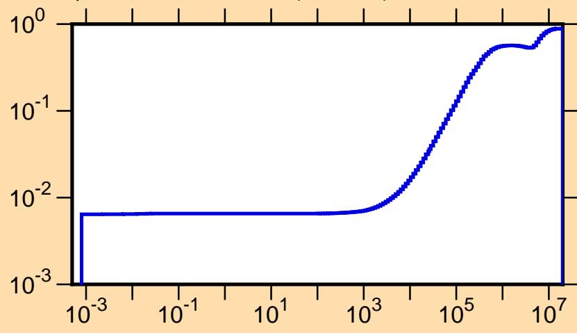
\mu vs. E for ^{105}\text{Mo}(\text{mt251})
