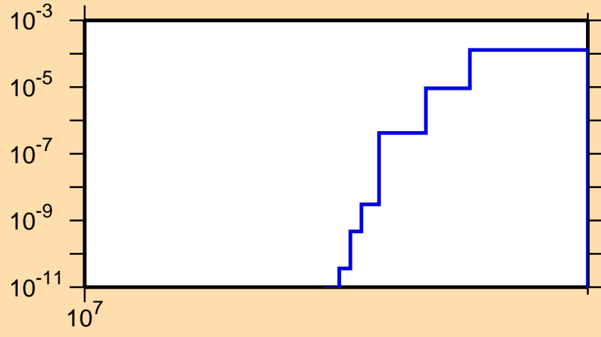
\sigma vs. E for ^{105}\text{Mo}(n,np)
