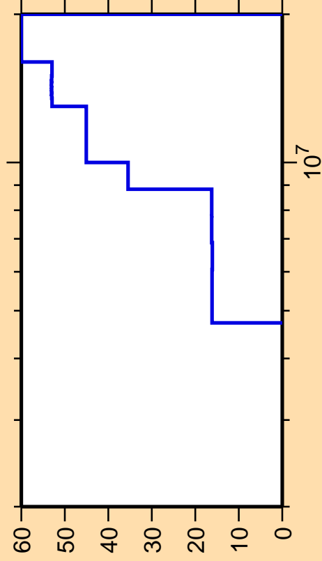
\Delta\sigma/\sigma vs. E for ^{105}\text{Mo}(n,2n)
