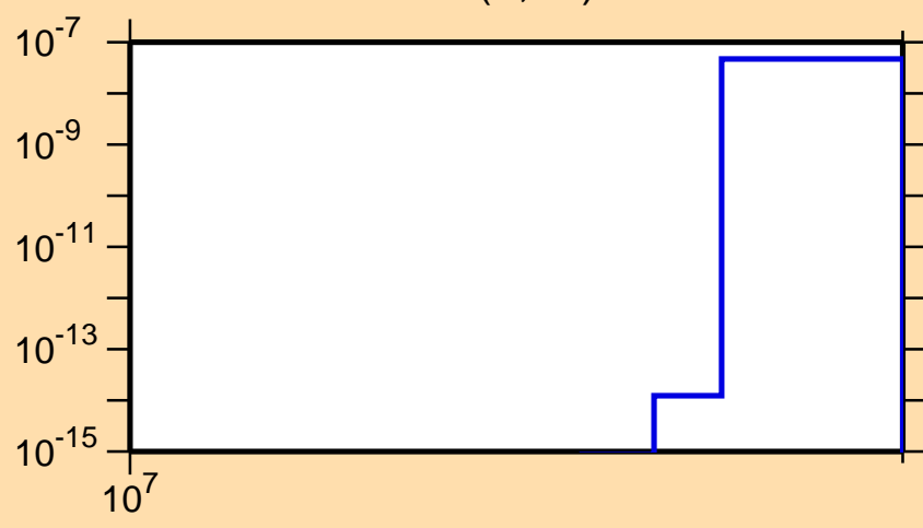
\sigma vs. E for ^{105}\text{Mo}(n,\text{nd})
