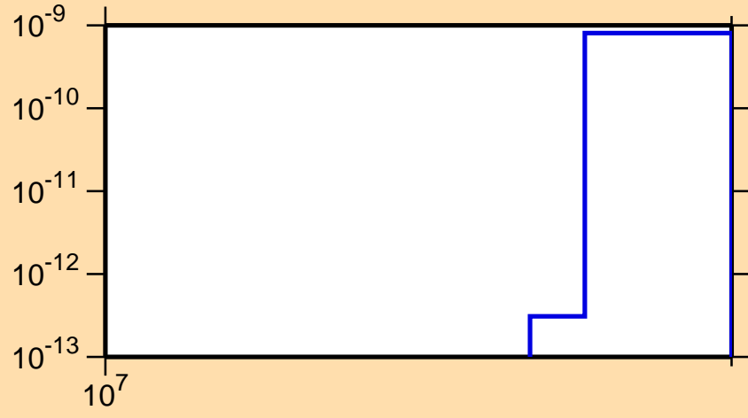
\sigma vs. E for ^{105}\text{Mo}(n,2n\alpha)
