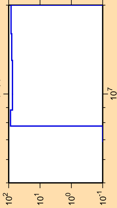
\Delta\sigma/\sigma vs. E for ^{105}\text{Mo}(n,p)
