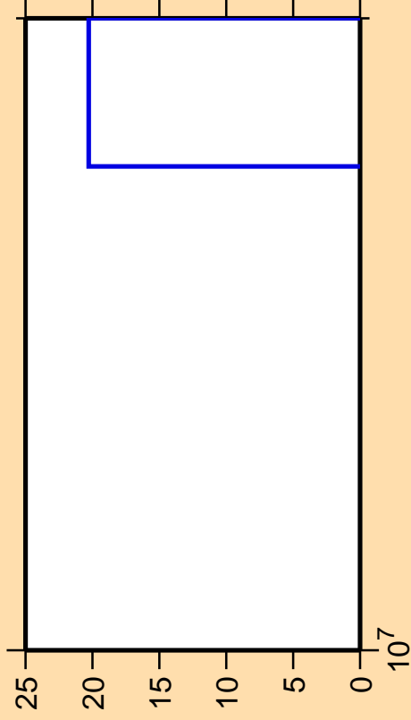
\Delta\sigma/\sigma vs. E for ^{105}\text{Mo}(n,2np)
