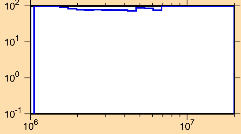
\Delta\sigma/\sigma vs. E for ^{105}\text{Mo}(n,n\text{cont.})
