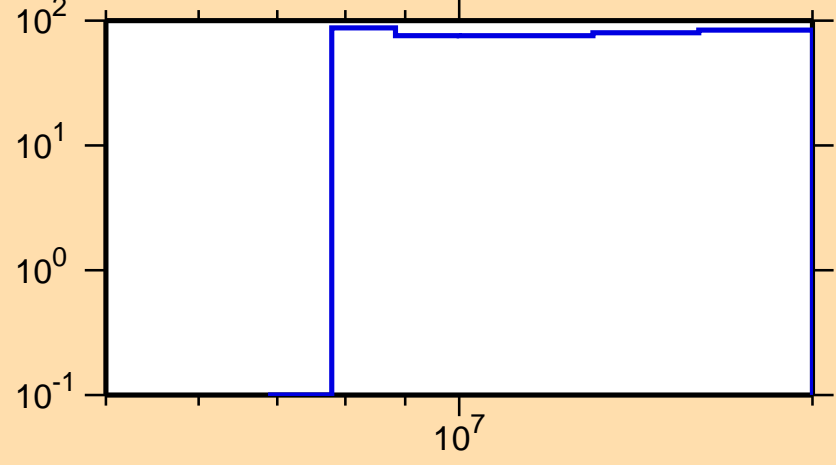
\Delta\sigma/\sigma vs. E for ^{105}\text{Mo}(n,p)
