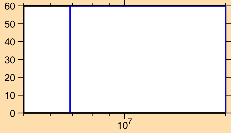
\Delta\sigma/\sigma vs. E for ^{105}\text{Mo}(n,ncont.)
