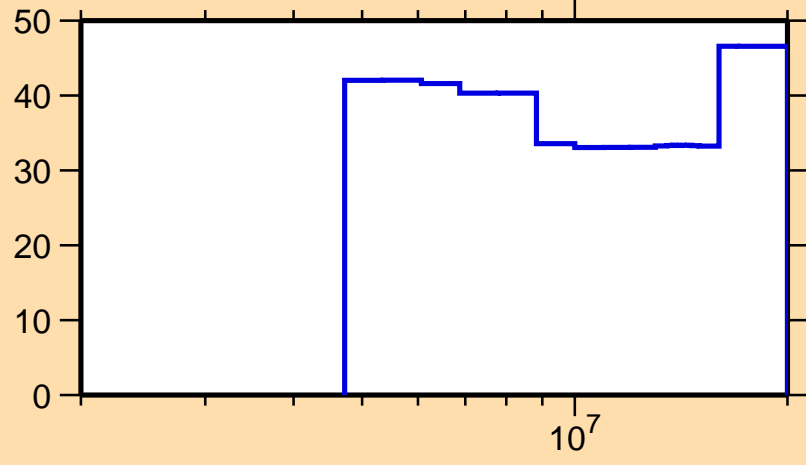
\Delta\sigma/\sigma vs. E for ^{105}\text{Mo}(n,\text{inel.})
