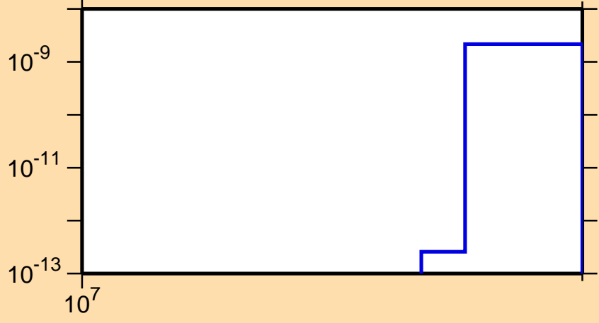
\sigma vs. E for ^{105}\text{Mo}(n,nt)
