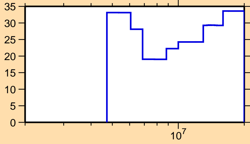
\Delta\sigma/\sigma vs. E for ^{105}\text{Mo}(n,\text{el.})
