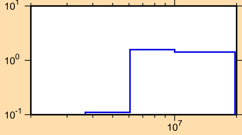
\sigma vs. E for ^{105}\text{Mo}(n,2n)
