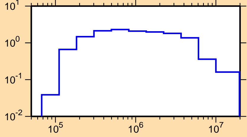
\sigma vs. E for ^{105}\text{Mo}(n,\text{inel.})
