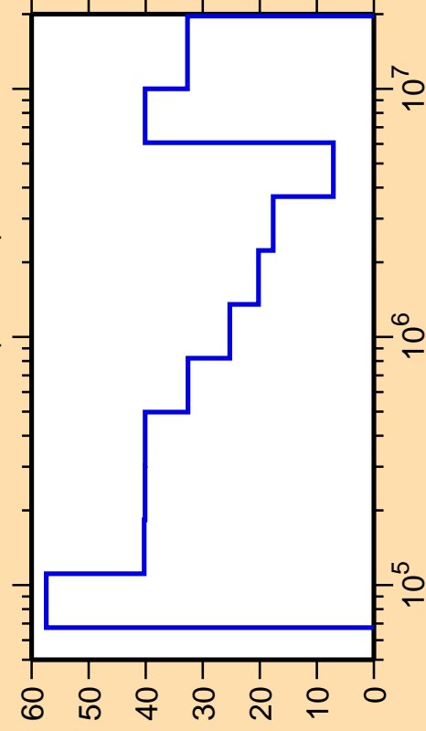
\Delta\sigma/\sigma vs. E for ^{105}\text{Mo}(n,\text{inel.})
