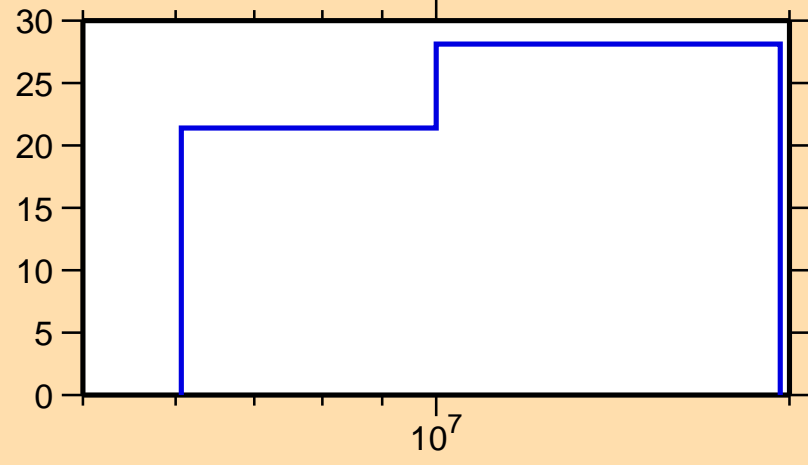
\Delta\sigma/\sigma vs. E for ^{105}\text{Mo}(n,el.)
