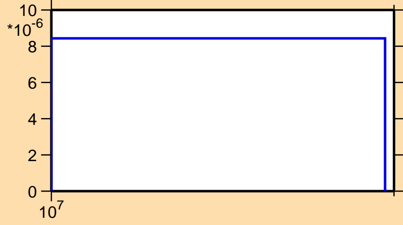
\sigma vs. E for ^{105}\text{Mo}(n,d)
