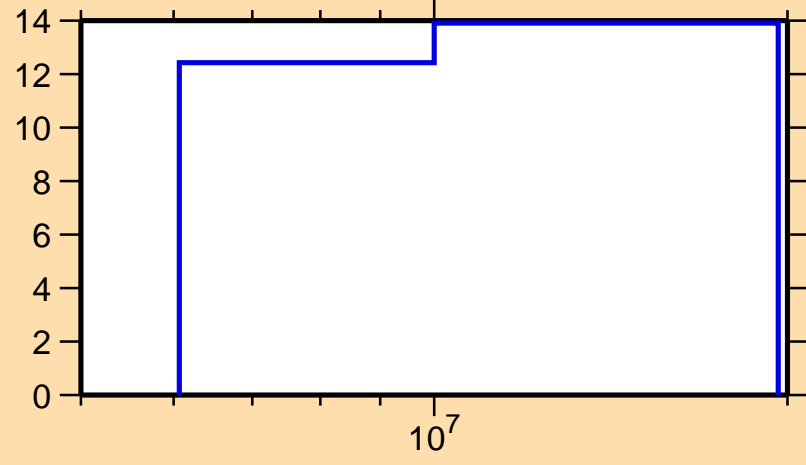
\Delta\sigma/\sigma vs. E for ^{105}\text{Mo}(n,\text{nonel.})
