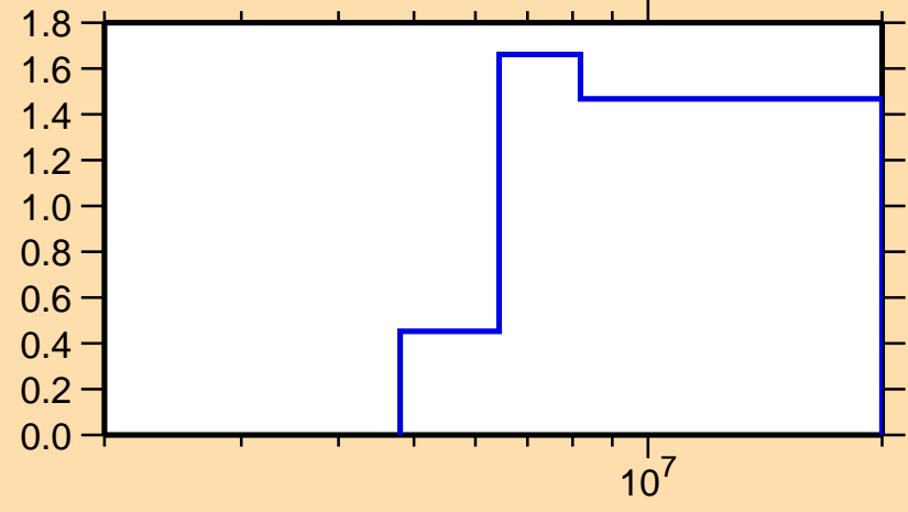
\sigma vs. E for ^{105}\text{Mo}(n,2n)
