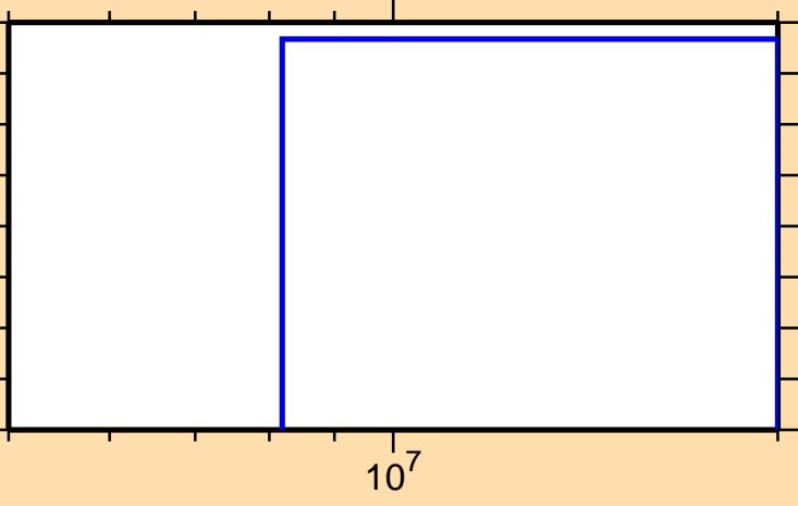
\sigma vs. E for ^{105}\text{Mo}(n,\text{nd})
