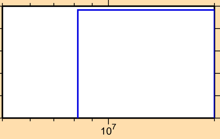
\sigma vs. E for ^{105}\text{Mo}(n,n\alpha)
