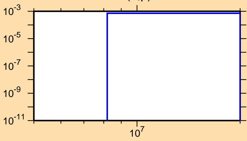
\sigma vs. E for ^{105}\text{Mo}(n,p)
