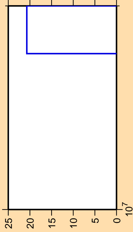
\Delta\sigma/\sigma vs. E for ^{106}\text{Mo}(n,\text{nd})
