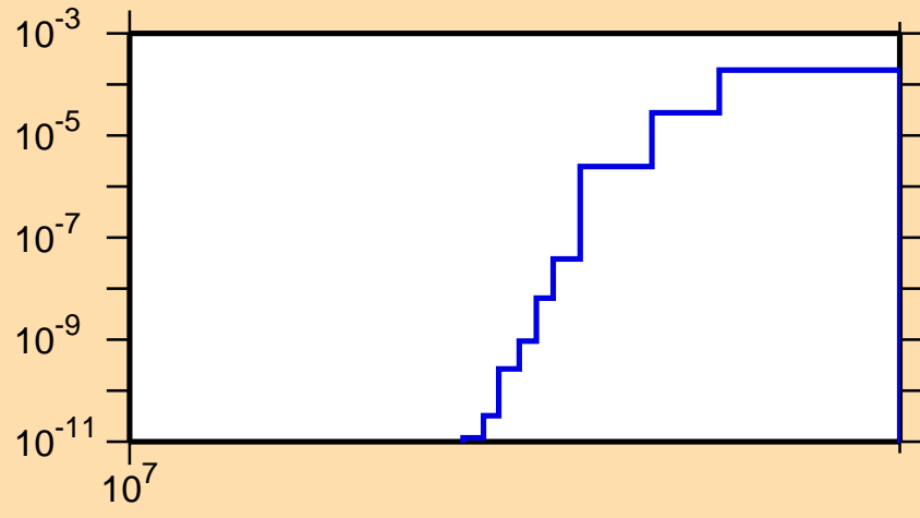
\sigma vs. E for ^{107}\text{Mo}(n,d)
