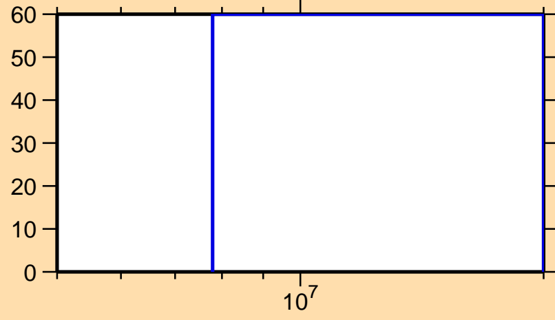
\Delta\sigma/\sigma vs. E for ^{107}\text{Mo}(n,\text{inel.})
