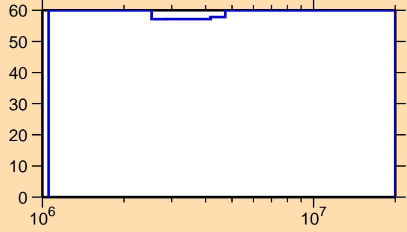
\Delta\sigma/\sigma vs. E for ^{107}\text{Mo}(n,n\text{cont.})
