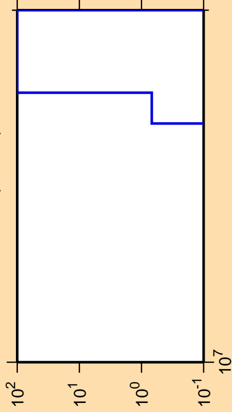
\Delta\sigma/\sigma vs. E for ^{107}\text{Mo}(n,2n\alpha)
