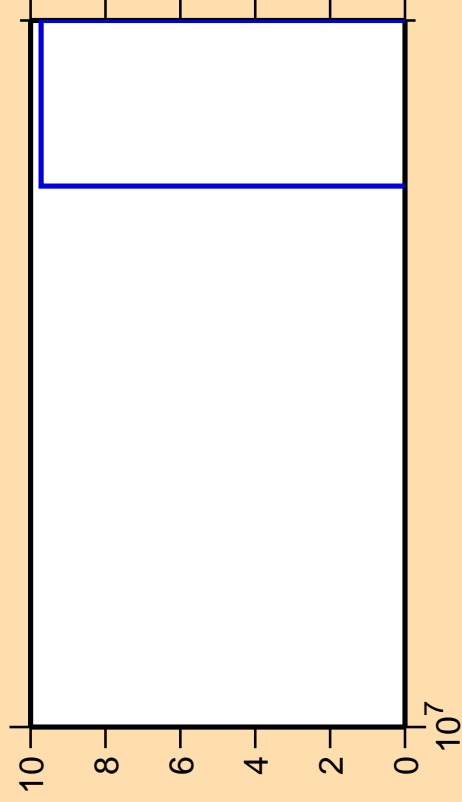
\Delta\sigma/\sigma vs. E for ^{107}\text{Mo}(n,2np)
