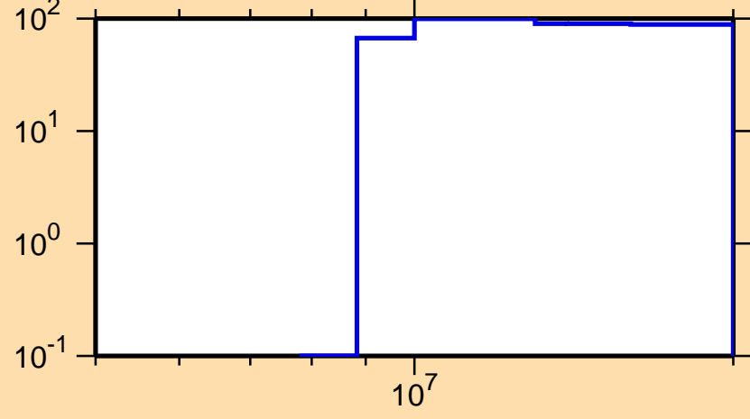
\Delta\sigma/\sigma vs. E for ^{107}\text{Mo}(n,p)
