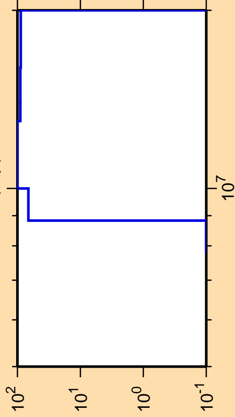
\Delta\sigma/\sigma vs. E for ^{107}\text{Mo}(n,p)
