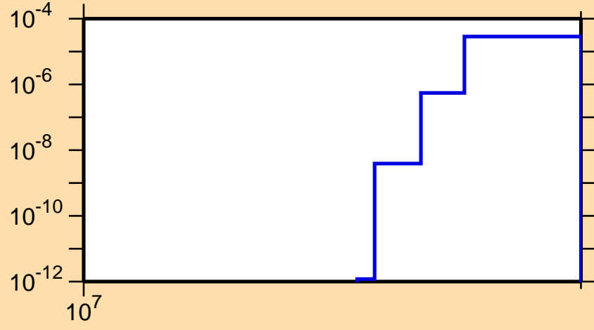
\sigma vs. E for ^{107}\text{Mo}(n,np)
