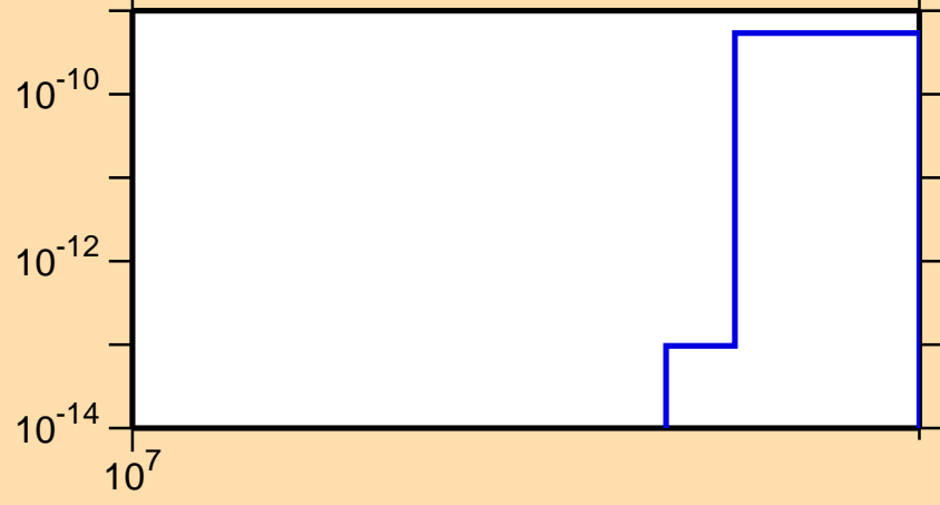
\sigma vs. E for ^{107}\text{Mo}(n,2n\alpha)
