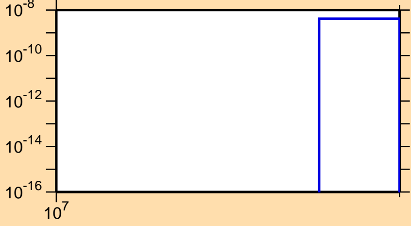
\sigma vs. E for ^{107}\text{Mo}(n,nt)
