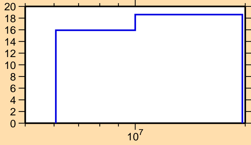
\Delta\sigma/\sigma vs. E for ^{107}\text{Mo}(n,el.)
