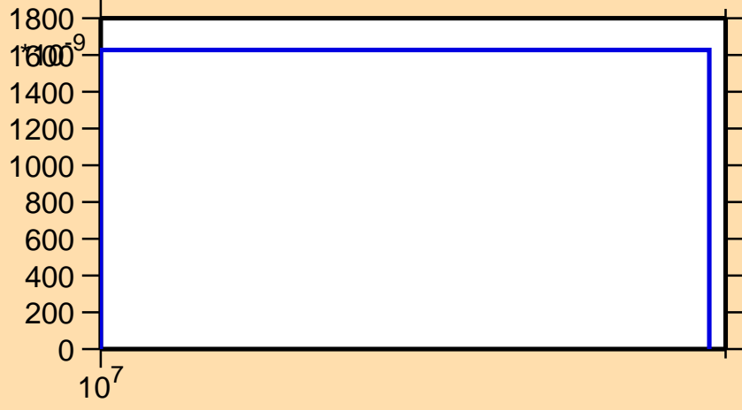
\sigma vs. E for ^{107}\text{Mo}(n,t)
