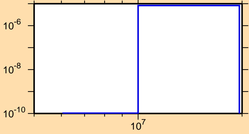
\sigma vs. E for ^{107}\text{Mo}(n,\alpha)
