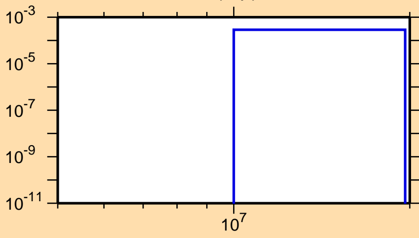
\sigma vs. E for ^{107}\text{Mo}(n,p)
