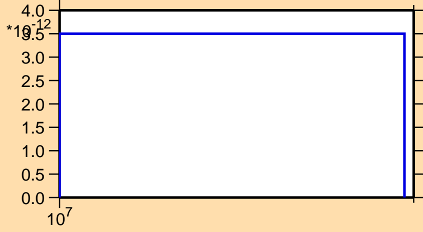
\sigma vs. E for ^{107}\text{Mo}(n,2n\alpha)
