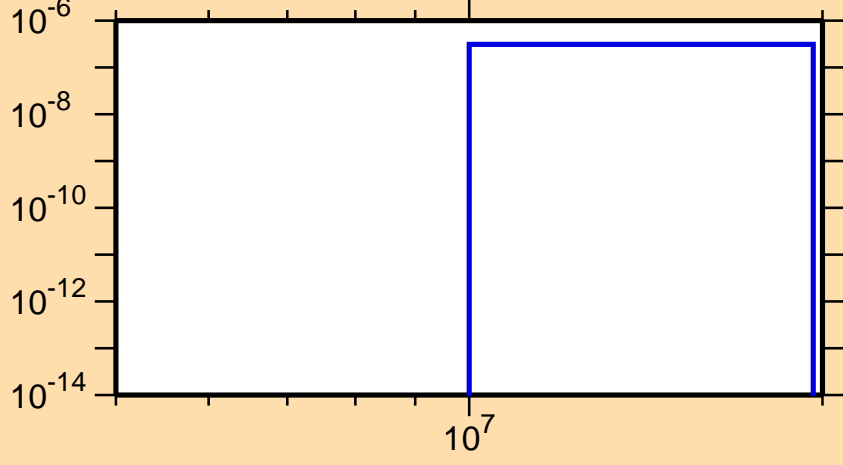
\sigma vs. E for ^{107}\text{Mo}(n,n\alpha)
