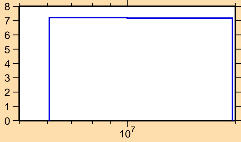
\Delta\sigma/\sigma vs. E for ^{107}\text{Mo}(n,\text{tot.})
