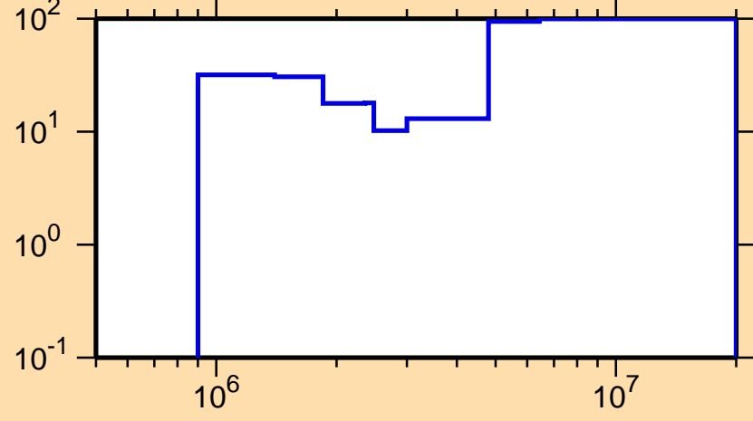
\Delta\sigma/\sigma vs. E for ^{107}\text{Mo}(n,\text{inel.})
