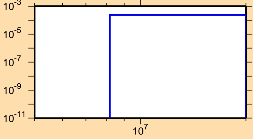
\sigma vs. E for ^{107}\text{Mo}(n,p)
