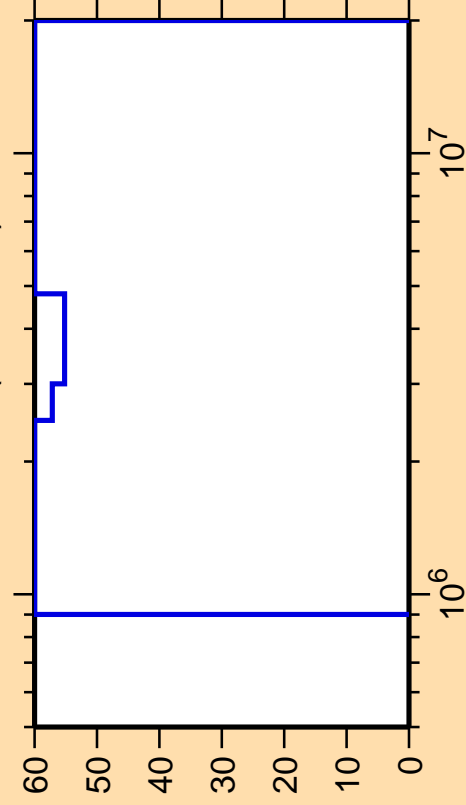
\Delta\sigma/\sigma vs. E for ^{107}\text{Mo}(n,n\text{cont.})
