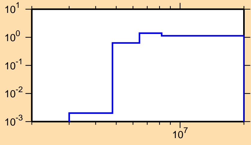
\sigma vs. E for ^{107}\text{Mo}(n,2n)
