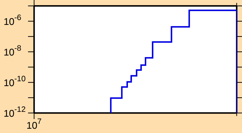
\sigma vs. E for ^{108}\text{Mo}(n,n\alpha)
