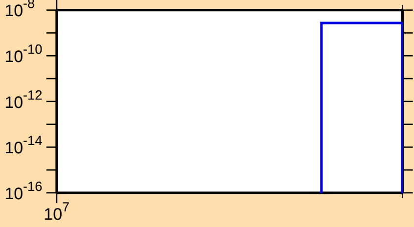
\sigma vs. E for ^{108}\text{Mo}(n,\text{nt})
