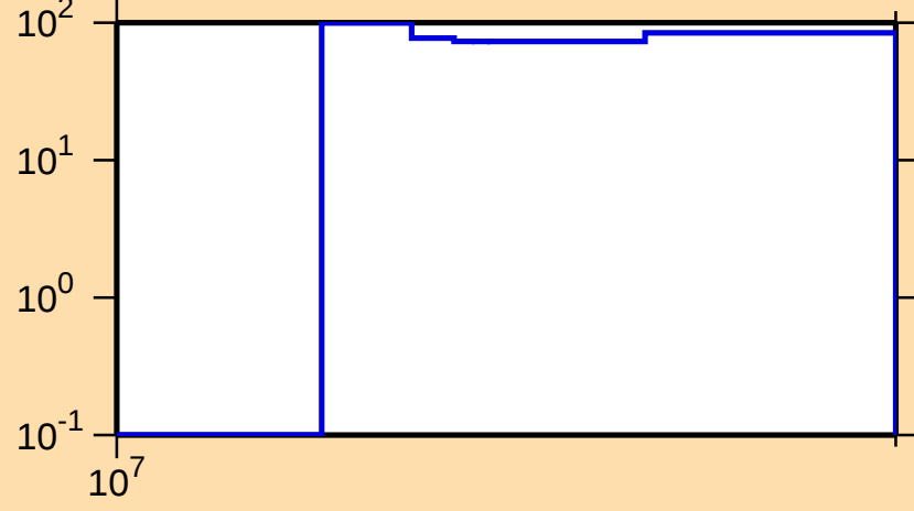
\Delta\sigma/\sigma vs. E for ^{108}\text{Mo}(n,p)
