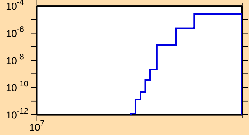
\sigma vs. E for ^{108}\text{Mo}(n,t)
