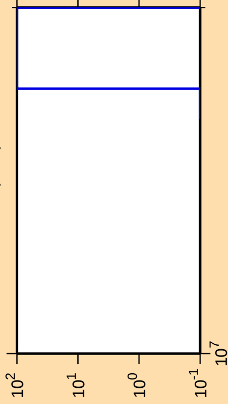
\Delta\sigma/\sigma vs. E for ^{108}\text{Mo}(n,\text{nt})
