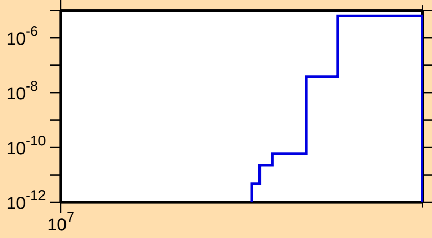
\sigma vs. E for ^{108}\text{Mo}(n,np)
