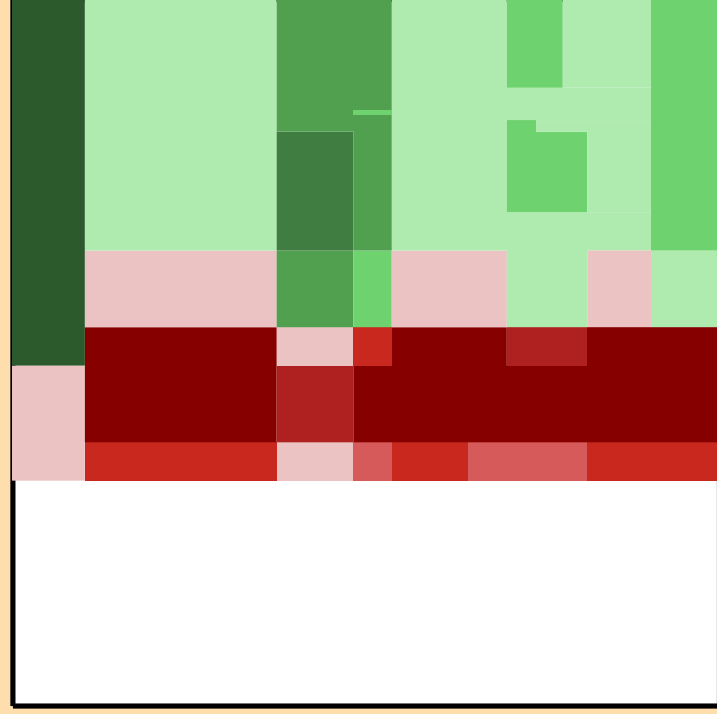
\Delta\sigma/\sigma vs. E for ^{108}\text{Mo}(n,n_1)
