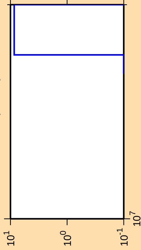
\Delta\sigma/\sigma vs. E for ^{108}\text{Mo}(n,2n\alpha)
