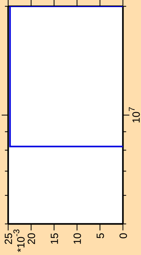
\Delta\sigma/\sigma vs. E for ^{108}\text{Mo}(n,\text{nd})
